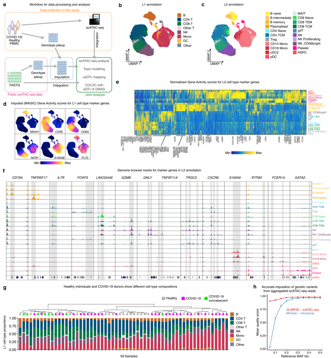
960 961 Fig. 1. An integrated map of scATAC-seq of PBMC from 20 donors with active COVID-19, 962 19 COVID-19 convalescent donors and 20 healthy controls. a , Schematic representation of 963 sample collection, data integration and analysis workflow. (Some icons are from bioicons.com). 964 b , A UMAP embedding of all cells from three integrated studies, colored by Azimuth L1 annotation 965 of seven common immune cell-types. c , The same UMAP embedding as in b , colored by 21 966 immune cell-types and subtypes in Azimuth L2 annotation. d , Gene activity scores of marker 967 genes in the seven common immune cell-types. Scores were imputed with MAGIC for 968 visualization purposes. e , Heatmap for marker genes for cell subtypes in L2 annotation. f , Color- 969 coded genome browser tracks of aggregated scATAC-seq reads in genomic loci around marker
