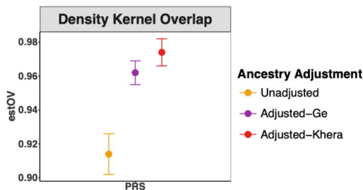
Figure 3. Effects of post hoc ancestry adjustment on the overlap of PRS-CSx (meta option)
