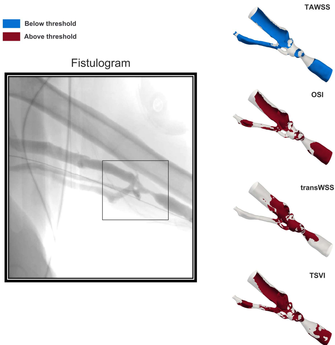
Figure 8. A 4-month follow-up fistulogram image of the cephalic vein region identified critical areas at the same location by the different near-wall hemodynamic indices. The transWSS index best co-localised qualitatively with the observed occlusion.
