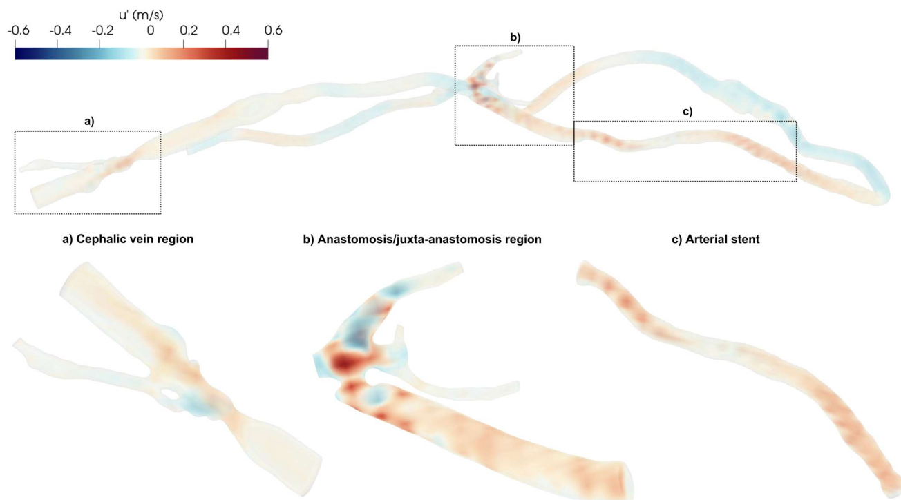
Figure 4. Velocity fluctuations of the x-component ( u' ) at peak systole in the whole domain and ROIs.
