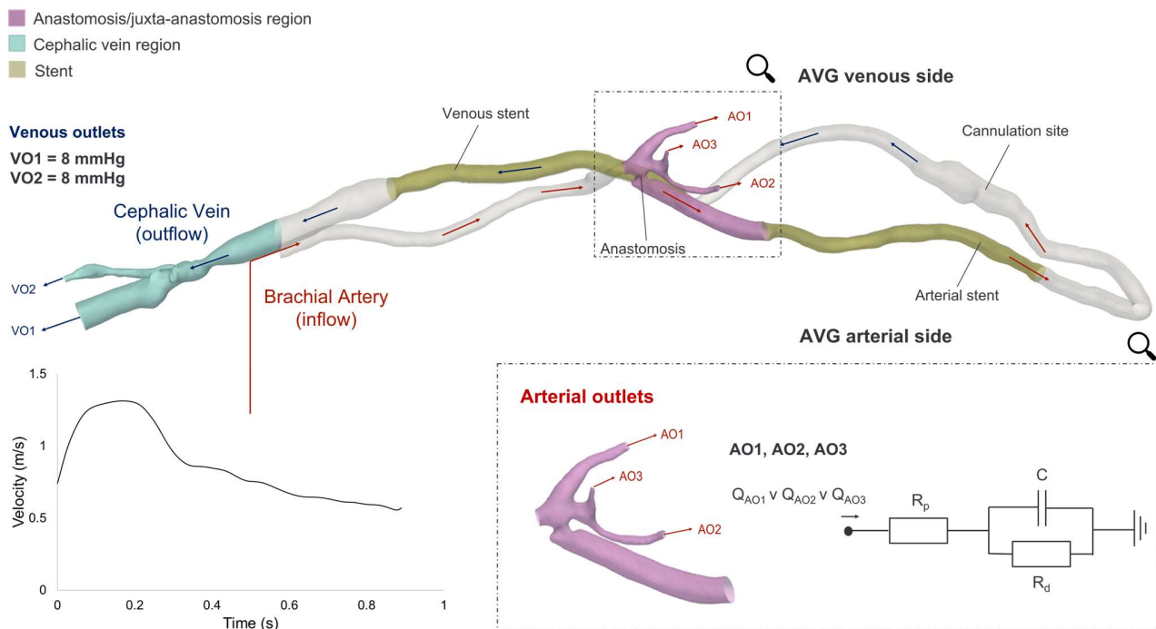
Figure 1. 3D reconstructed patient-specific computational domain. The arrows indicate blood flow direction and distinguish between arterial (red) and venous (blue) pathways. The manually extracted patient’s DUS velocity waveform was applied as inlet boundary condition at the brachial artery. Three-element Windkessel models were implemented at the arterial outlets of the domain (AO1, AO2 and AO3), and their parameters ( R_p , R_d and C ) were calibrated through a lumped-parameter 0D model of the computational domain. Q_{AO1} , Q_{AO2} and Q_{AO3} refer to the flow rates through the respective outlets determined by their respective cross-sectional areas. A static pressure of 8 mmHg was imposed at the venous outlets (VO1 and VO2).
