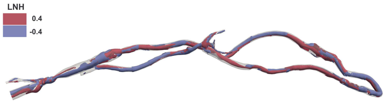
Figure 6. Cycle-averaged LNH in the whole computational domain. Blue and red colours indicate left-handed and right-handed helical flow rotation, respectively.
