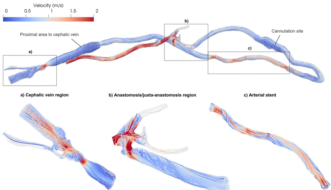
Figure 3. Velocity streamlines at peak systole in the whole domain and ROIs.
