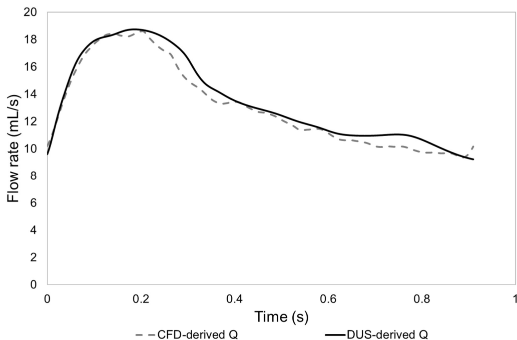
Figure 2. Flow waveforms derived from the DUS image (DUS-derived Q) and obtained from the CFD simulation (CFD-derived Q) at the proximal edge of the arterial stent.
