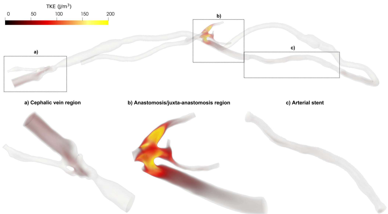
Figure 5. Volume rendering of TKE at peak systole for the whole domain and ROIs.
