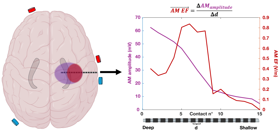
Figure S6. Recorded AM amplitude and calculated AM EF along an sEEG electrode targeting the hippocampus.
