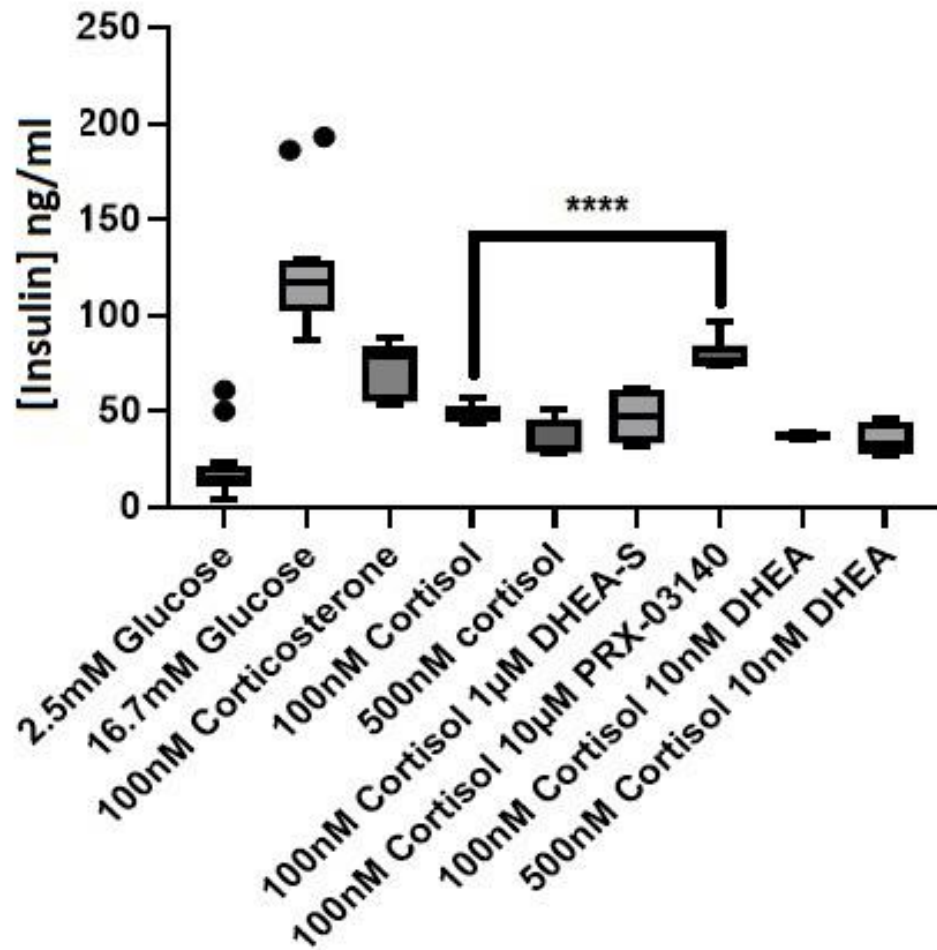
477 478 Figure 3: Response of INS-1 832/13 Cells to Corticosterone, Cortisol, Cortisol with PRX- 479 3140, DHEA and DHEA-S. After an 18 hours incubation with the test compounds, cells were 480 washed, starved for 1 hour with 2.5 mM glucose and then exposed for 2 hours with the test 481 compounds diluted in 16.7 mM glucose. The insulin content in the supernatant was determined 482 by ELISA. Each condition was tested at least 4 times. Data was analyzed using GraphPad Prism 483 using the Box and Whiskers plot (solid circles denote outliers.) **** Comparison of 100 nM 484 cortisol to 100nM cortisol with 10 µM PRX-3140; P<0.0001; Student's T test.
