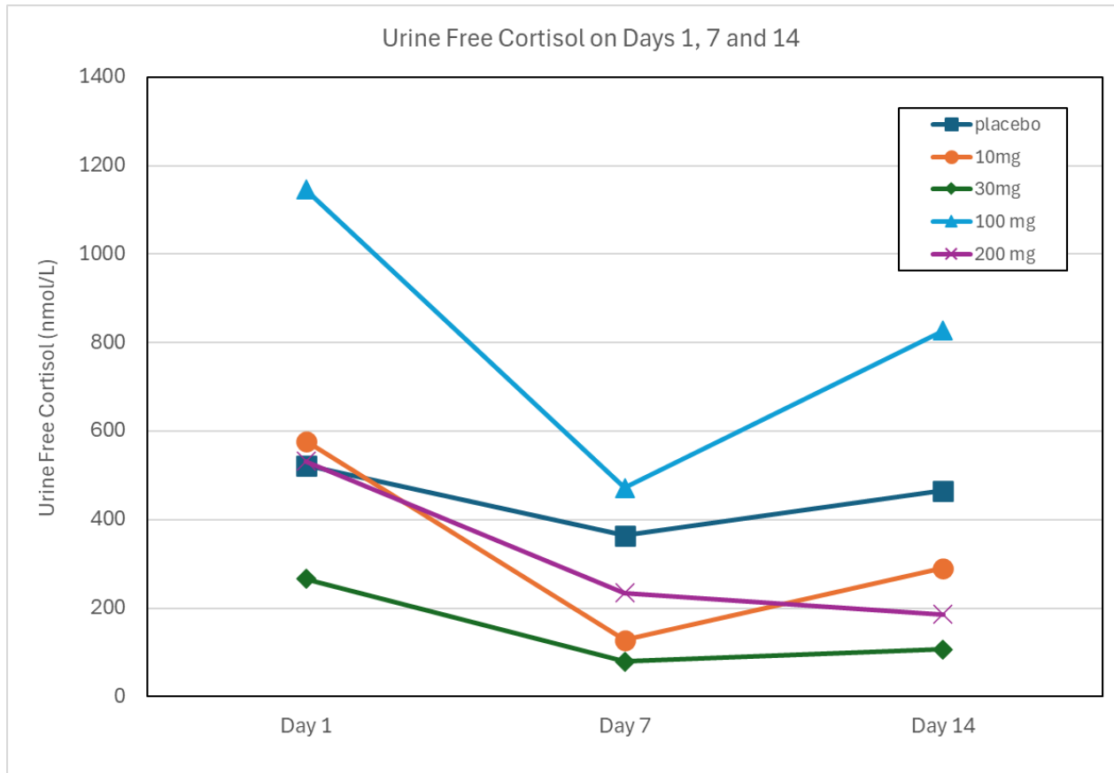
531 Figure 6: Urine Free Cortisol on Days 7 and 14. Urine Free Cortisol in Subjects pre-dose on 532 Day 1, 7 and Day 14 with oral administration of 10 mg (n=6), 30 mg (n=6), 100 mg (n=6), 200 mg 533 (n=6) PRX-03140 or Placebo (n=8) for 14 days.
