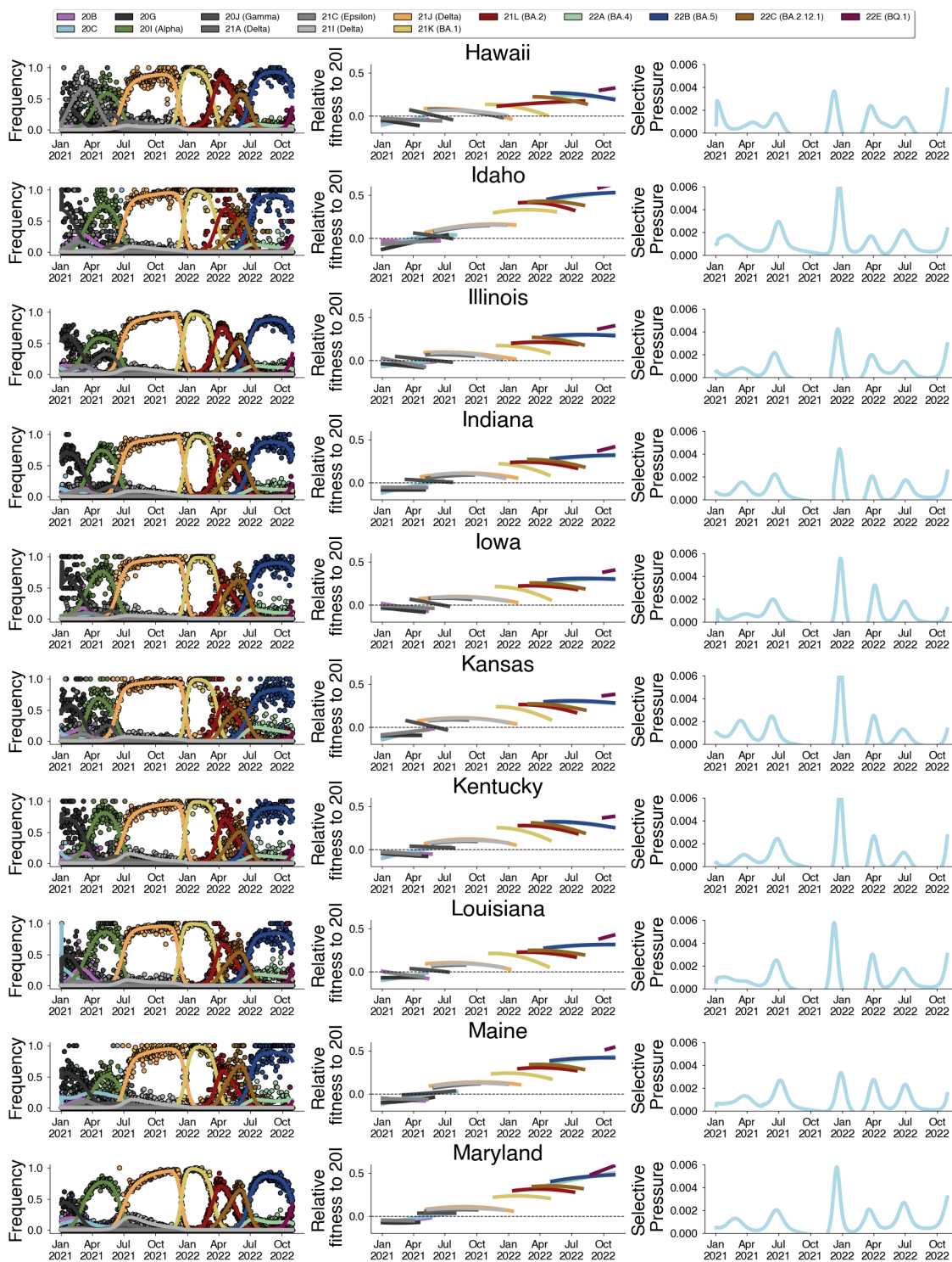
Fig. S4. Estimated variant frequencies, relative fitnesses, and selective pressure. Hawaii to Maryland.
