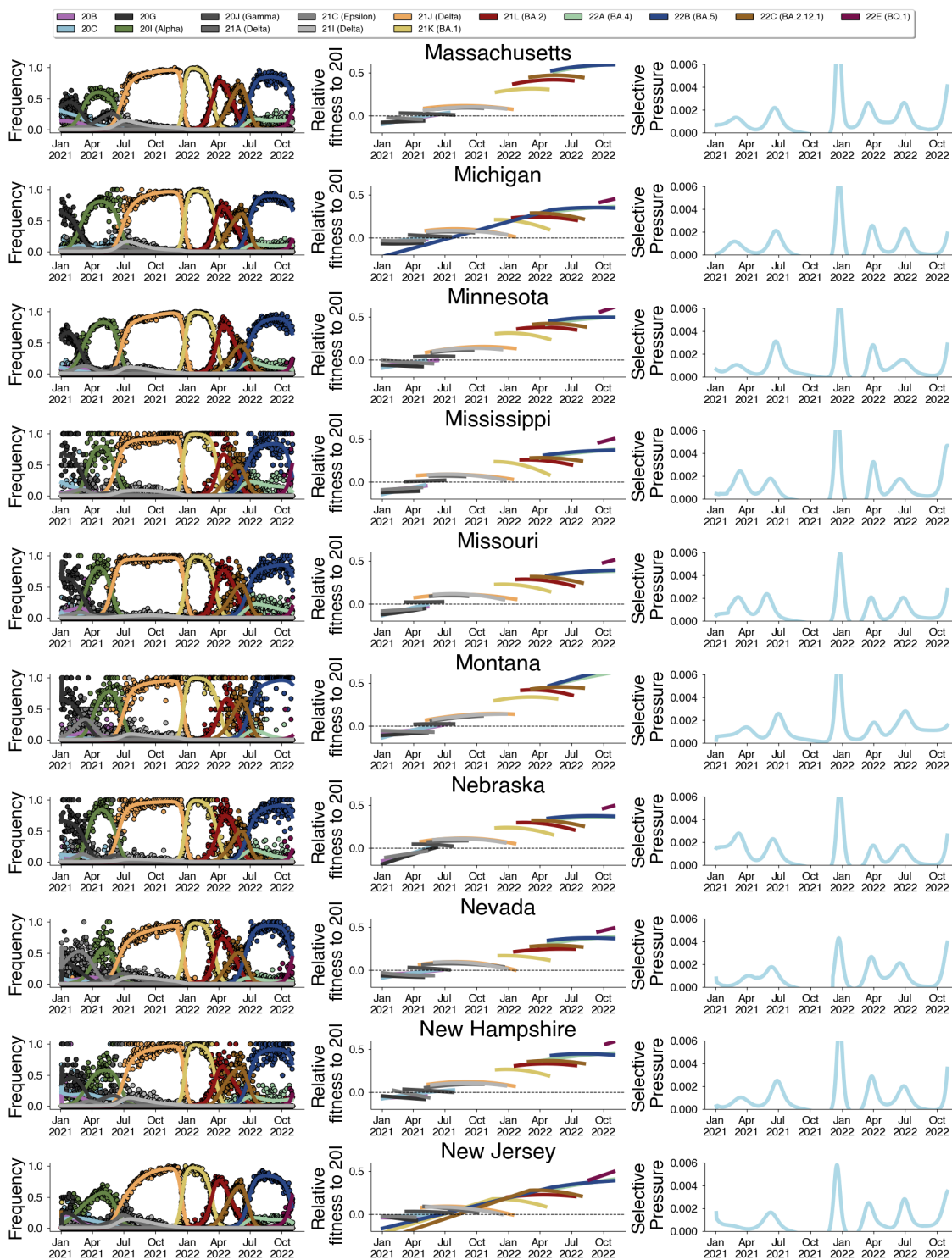
Fig. S5. Estimated variant frequencies, relative fitnesses, and selective pressure. Massachusetts to New Jersey.
