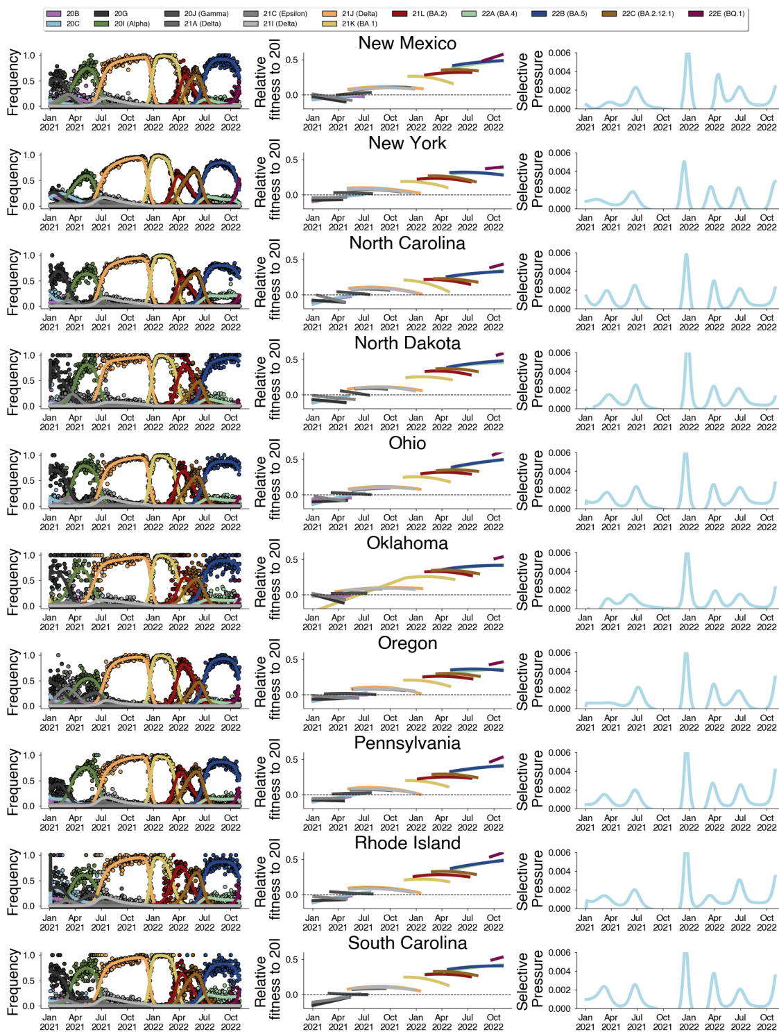
Fig. S6. Estimated variant frequencies, relative fitnesses, and selective pressure. New Mexico to South Carolina.
