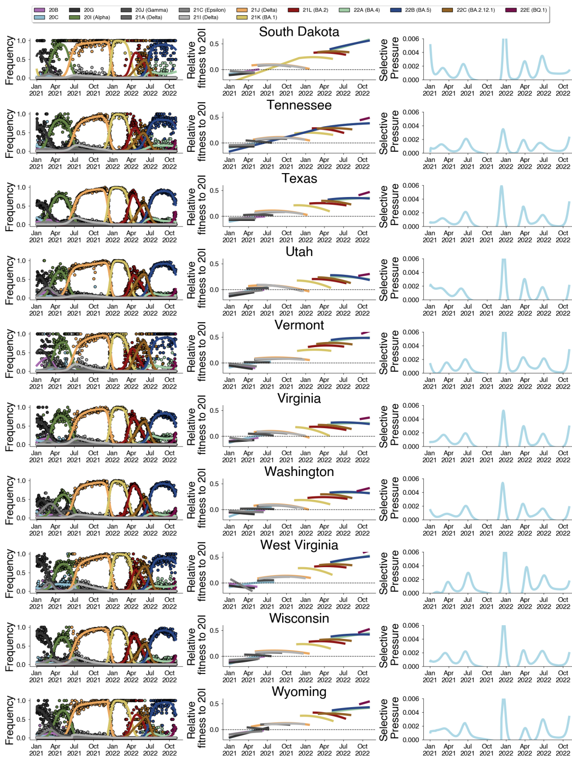
Fig. S7. Estimated variant frequencies, relative fitnesses, and selective pressure. South Dakota to Wyoming.
