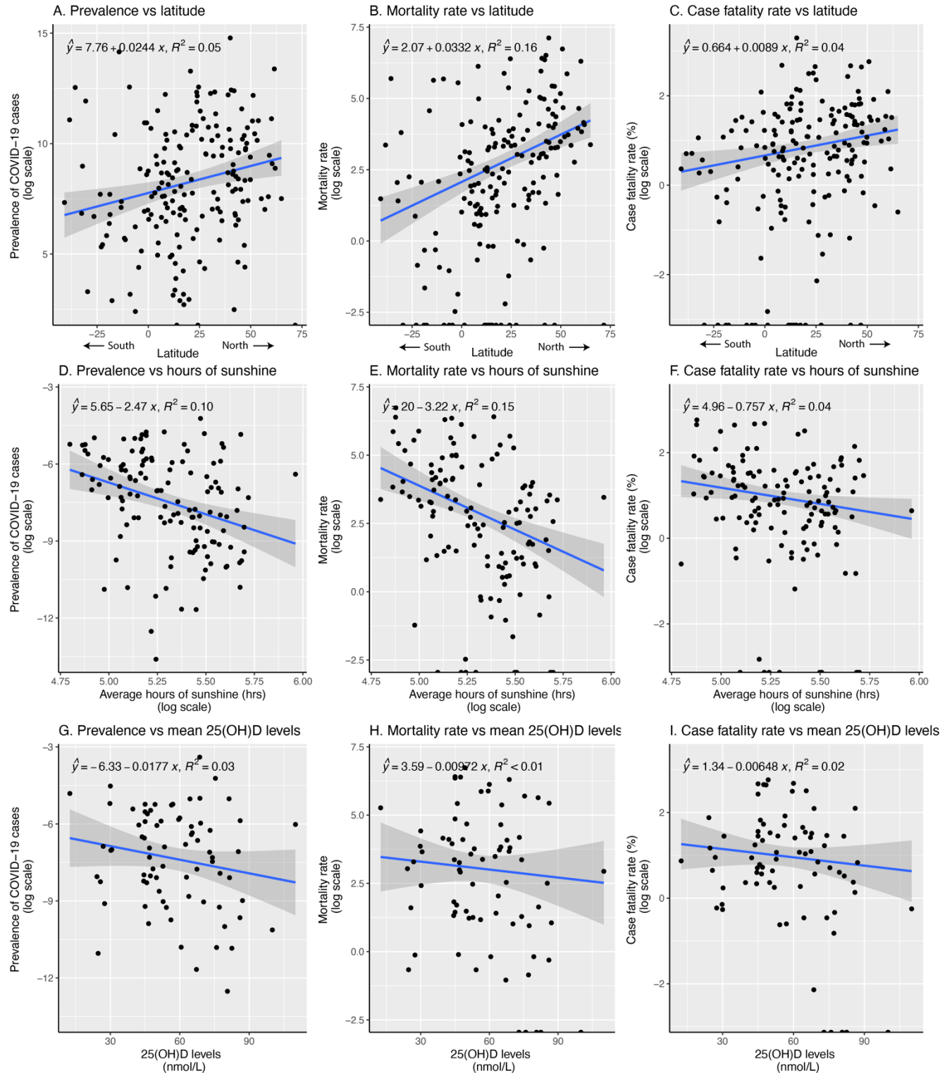
Figure 2. Correlations between COVID-19 metrics and environmental factors across countries. Each point on the plots represents data for an individual country. The COVID-19 prevalence is defined as the total number of reported cases per 1 million population, the mortality rate as the number of deaths per 1 million population, and the case fatality rate as the percentage of reported cases resulting in death, multiplied by 100.
