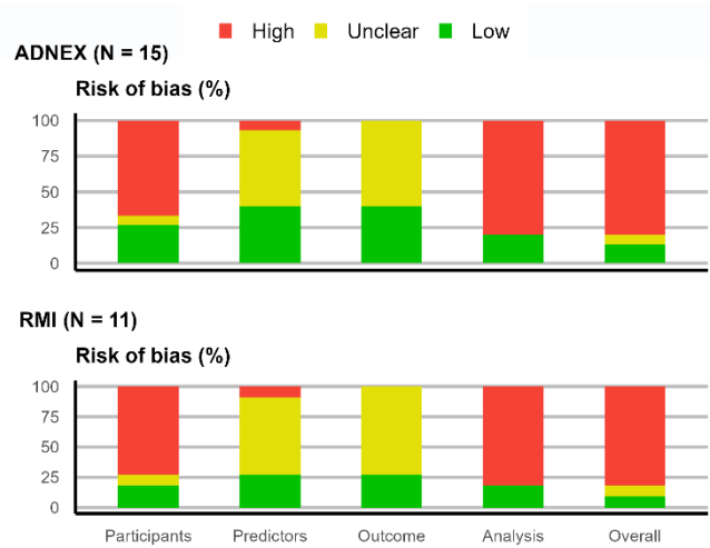
Fig. 1: Risk of bias by subdomain and overall for Assessment of Different NEoplasias in the adneXa (ADNEX) and Risk of malignancy index (RMI) validations using the Prediction model Risk Of Bias ASsessment Tool (PROBAST). There are 15 validations of ADNEX and 11 validations of RMI.
