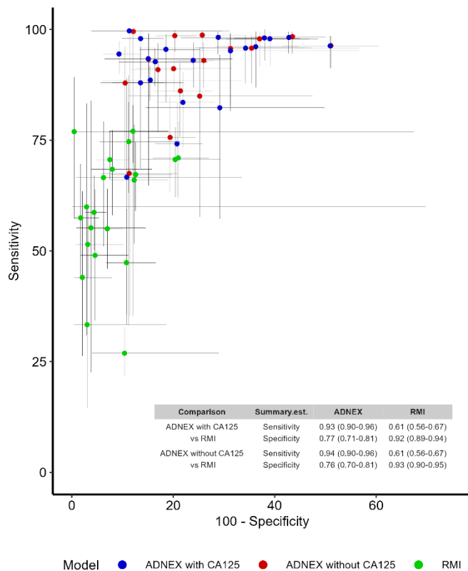
Fig. 3: Sensitivity and specificity of ADNEX (10% cutoff) and RMI (cutoff 200) in surgically managed patients illustrated in the space of a receiver operating characteristic curve. Each point represents the result of one study or centre and the lines represent the 95% confidence interval.
