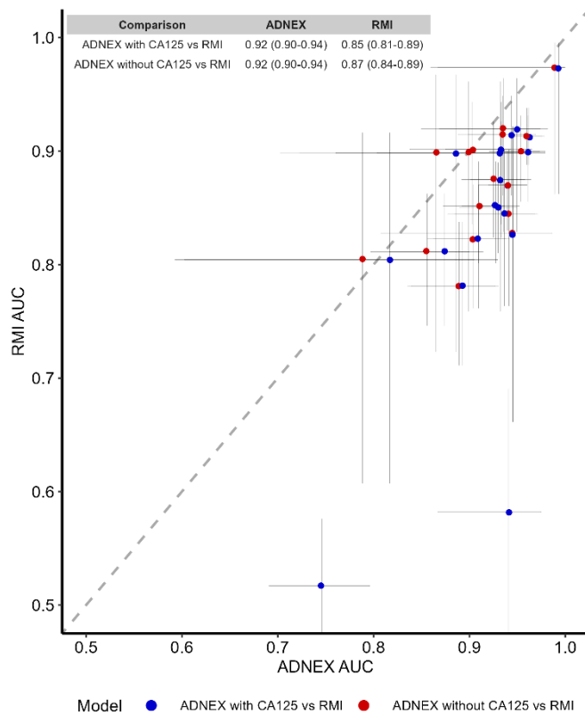
Fig. 2: Comparison of the area under the receiver operating characteristic curve (AUC) of ADNEX (with and without CA125) and RMI per centre in the included studies for only operated patients. Vertical and horizontal lines present the confidence interval of each centre's AUC. Dots below the diagonal line indicate higher AUC for ADNEX than for RMI. Dots above the diagonal line indicate higher AUC for RMI.
