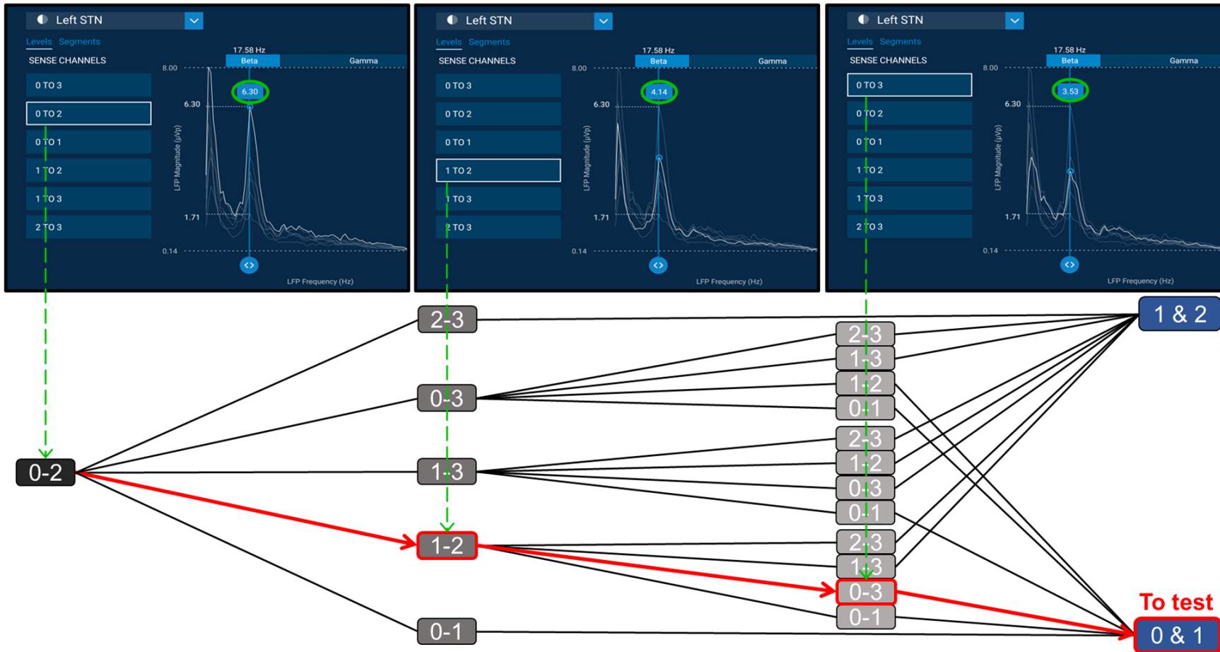
Figure 2. Example of the “selection decision tree” online ranking technique which uses the two or three recording channels with the highest beta feature value to select the two most likely best contact-levels. For this method the clinician performs a BrainSense™ Survey for the contact-levels using the clinician programmer. These contact-level recordings can thereafter be used on-screen to visually select the channel (contact pair) with the highest beta peak (i.e. channel “0 to 2” in this example). This information is used to choose the appropriate “selection decision tree”, i.e. the one which starts with the selected channel. Hereafter, the channel with the second highest beta peak (here channel “1 to 2”) is selected in the first branch of the decision tree. Finally, the channel with the third highest beta peak (here channel “0 to 3”) is selected in the second and final branch. This then leads to a final block which shows which contact-levels are expected to be most promising (here level 0 and 1) based on the “selection decision tree” technique and should thus be considered (first) during the clinical contact-level evaluation.
