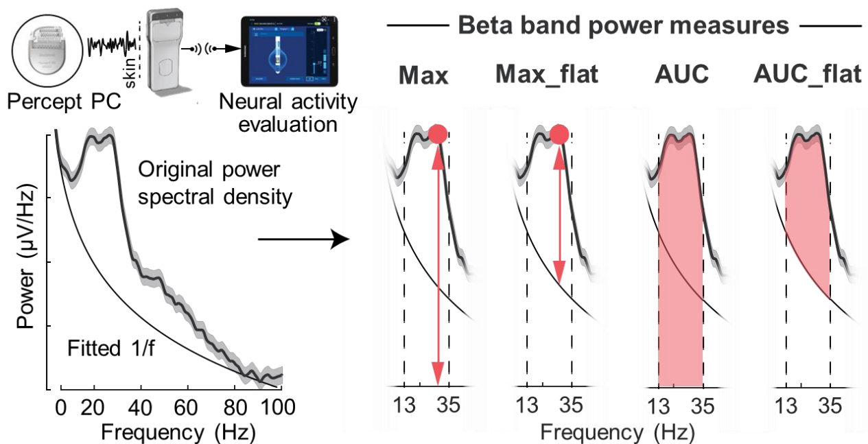
Figure 1. Original spectrum and FOOOF-algorithm aperiodic fit demonstrating the extraction of four beta-band power measures: the maximum power (Max); the maximum flattened (i.e. after removal of the aperiodic signal component) power (Max_flat); the area under the curve (AUC); and the flattened area under the curve (AUC_flat).
