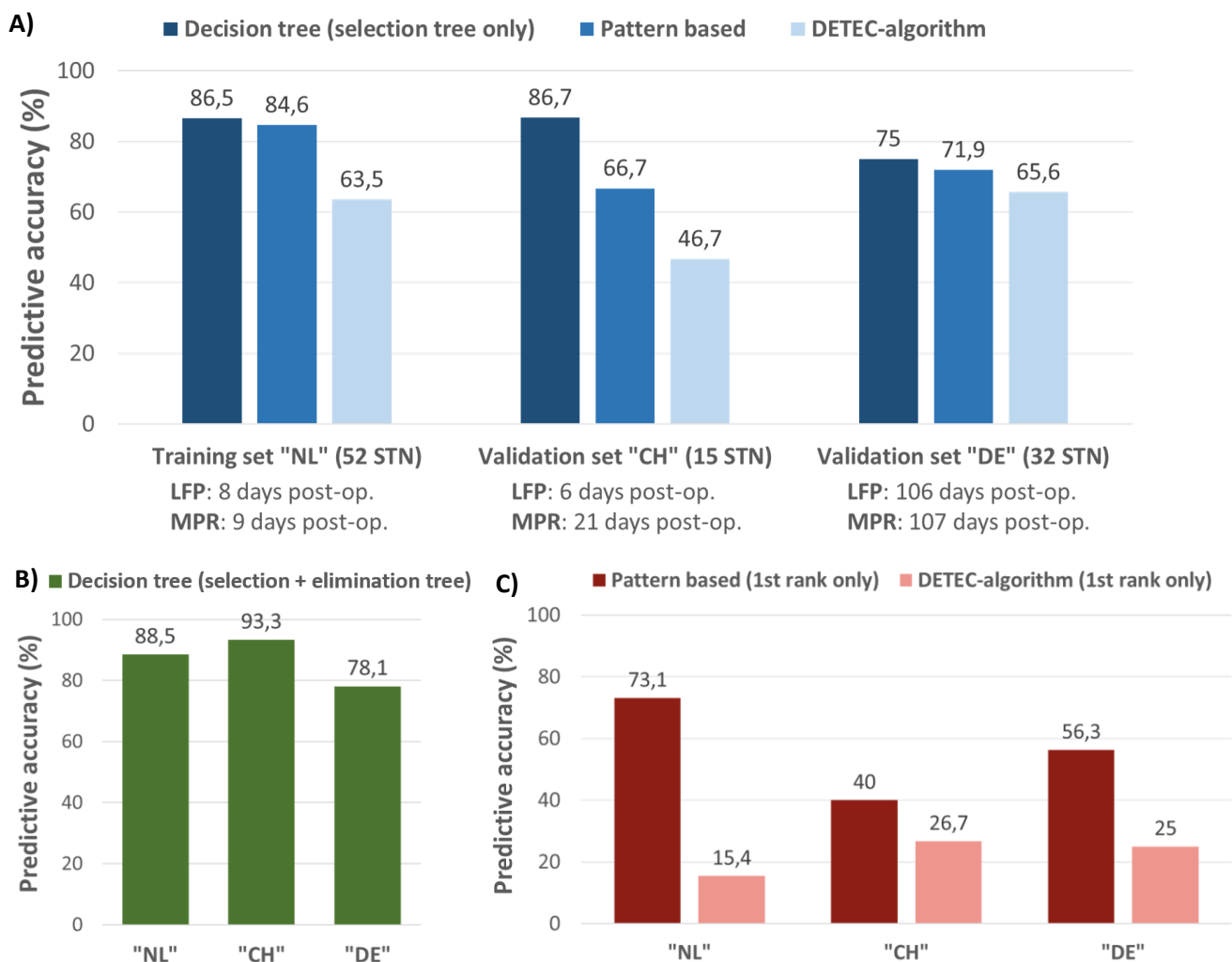
Figure 5. Comparison of algorithm performances when considering the results for the 1 st and 2 nd ranked contact-levels in recordings with clear beta activity obtained in OFF-medication. The time from the implant to LFP recordings (LFP: used for prediction) and the time from implant to the clinical contact selection (MPR: reference for prediction) varied between centres (see text). A) Predictive accuracy of the novel ‘decision tree – selection only’ and ‘pattern based’ prediction techniques for the ‘Max’ beta feature in comparison to the predictive accuracy of the existing DETEC-algorithm when considering both the 1 st and 2 nd ranked contact-levels. B) Predictive accuracy for the 1 st and 2 nd ranked contact-levels based on the online ‘decision tree’ method when applying the selection tree in combination with the elimination tree. C) Predictive accuracy of the offline “pattern based” method and DETEC-algorithms for the 1 st ranked contact-level alone.
