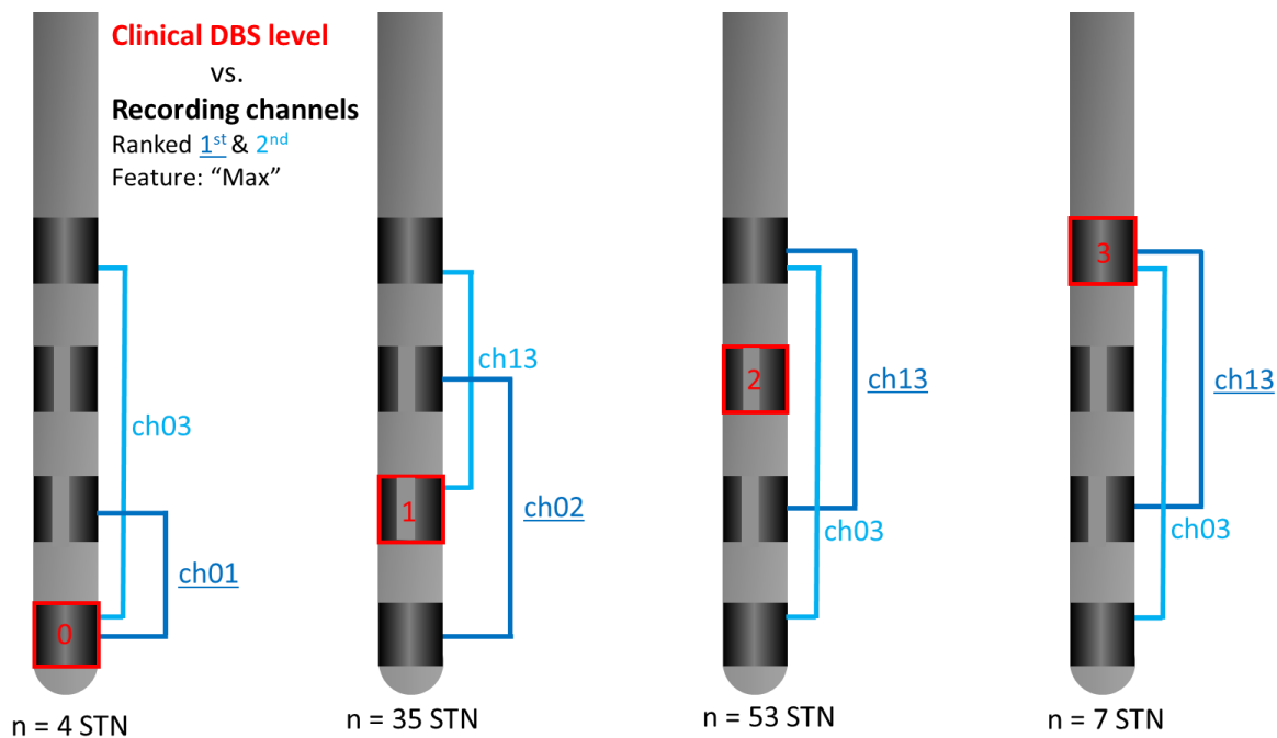
Figure 4. First- (dark blue) and second-ranked (light blue) recording channel (ch) per clinically chosen deep brain stimulation (DBS) contact-level at monopolar review (in red) for the maximal power beta-frequency band feature (“Max”). Results from all included leads with clear beta activity.
