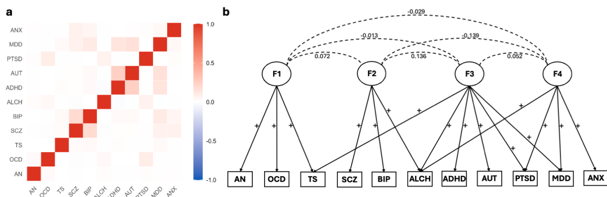
Figure 3: The genetic architecture and identified latent factor structures among eleven psychiatric disorders. a . Genetic correlation structure of the eleven disorders estimated using LDSC. b . Four latent psychiatric factors underlying the 11 disorders and their associations with the disorders inferred by genomicSEM. The four factors align well with four subtypes of psychiatric disorders, including compulsive, psychotic, neurodevelopmental, and internalizing disorders. The values on the dashed lines connecting each pair of factors are the between-factor correlations estimated by CaLMR (Multi). The signs near the solid lines linking factors with the observed disorders indicate the estimated signs of genetic correlations derived from genomicSEM. The signs reflect our known directions of the exposure-trait associations and will be used to determine the direction of the exposure-outcome effects. Abbreviations: AN (anorexia nervosa), OCD (obsessive-compulsive disorder), TS (Tourette syndrome), SCZ (schizophrenia), BIP (bipolar disorder), ALCH (problematic alcohol use), ADHD (attention-deficit/hyperactivity disorder), AUT (autism spectrum disorder), PTSD (post-traumatic stress disorder), MDD (major depressive disorder), ANX (anxiety).
