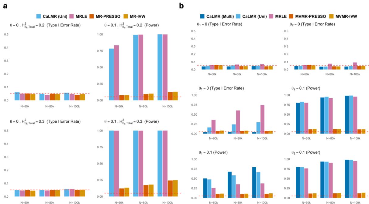
Figure 2: Simulation results under the single-exposure (a) and multiple-exposure (b) scenarios assuming a GWAS sample size for each trait and the outcome N = 60K, 80K, 100K . Results are summarized across 1000 simulations per setting. a. type I error control and power comparison between CaLMR (Uni), MRLE, MR-PRESSO, and MR-IVW under the single exposure setting. The significance threshold for IV selection is equal to p = 5 \times 10^{-4} . We assume the heritability of X is 0.2, and the total heritability of each biomarker H_{B_i, total}^2 = 0.2 (top panel) or 0.3 (bottom panel). b. type I error control and power comparison between CaLMR (Multi), CaLMR (Uni), MRLE, MV MR-PRESSO, and MV MR-IVW in the setting of two correlated latent exposures.
