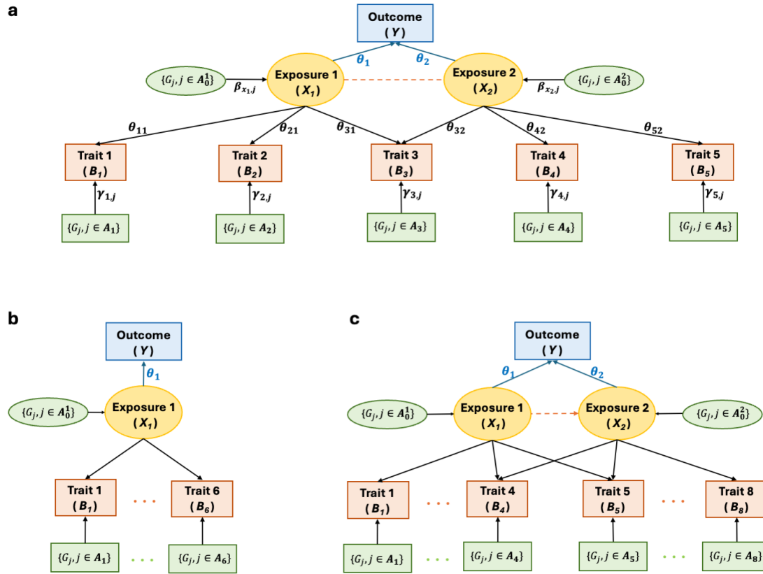
Figure 1: Causal diagrams illustrating the causal links between the outcome ( Y ), latent exposures ( X_1 and X_2 ), observable traits ( B_k ), and genetic IVs ( G_j ). a. An example causal diagram describing the general relationship between variables assumed by CaLMR in the two-exposure scenario. \theta_1 and \theta_2 are the parameters of interests, which are the causal effects of the latent exposures on Y . The red dashed line that links the two exposures indicates a potential between-exposure correlation. A_k denotes the set of SNPs associated with B_k and A_0^l the set of SNPs associated with latent exposure X_l . \gamma_{k,j} s and \beta_{x_l,j} s are the direct SNP effects on the observable traits and latent exposures, respectively. The existence of \theta_{31} and \theta_{32} reflects the case where some traits ( B_3 ) are regulated by multiple exposures. b. A causal diagram describing the single-exposure simulation setting assuming a total of K = 6 observable traits. c. An illustration of the multiple-exposure simulation setting assuming a total of eight observable traits co-regulated by two correlated latent exposures (correlation: \kappa = -0.5 ), among which two ( B_4 and B_5 ) are regulated by both exposures.
