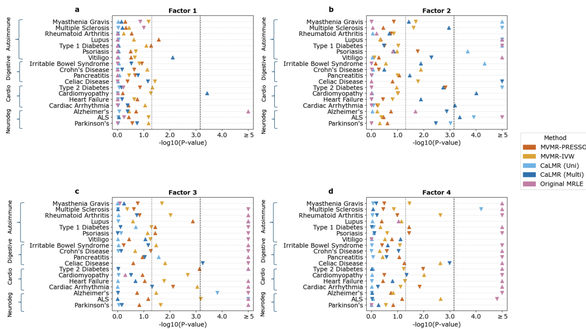
Figure 4: Analysis of Causal Effects of Psychiatric Factors on Various Disease Outcomes. We report the -\log_{10} p-values associated with testing the causal effects of four latent psychiatric factors on 18 disease outcomes using five methods, including MVMR-IVW, MVMR-PRESSO, MRLE, CaLMR (Uni), and CaLMR (Multi). Upward-pointing triangles represent positive causal estimates, whereas downward-pointing triangles represent negative estimates. The gray dashed line marks \alpha = 0.05 , and the black dashed line marks the adjusted significance level \alpha' = 0.0007 . Results are summarized by factor for Factor 1 (aligned with compulsive disorders, a ), Factor 2 (aligned with psychotic disorders, b ), Factor 3 (aligned with neurodevelopmental disorders, c ), and Factor 4 (aligned with internalizing disorders, d ). The eighteen disease outcomes include various autoimmune, digestive, cardiometabolic, and neurodegenerative disorders as indicated by the brackets on the y-axis.
