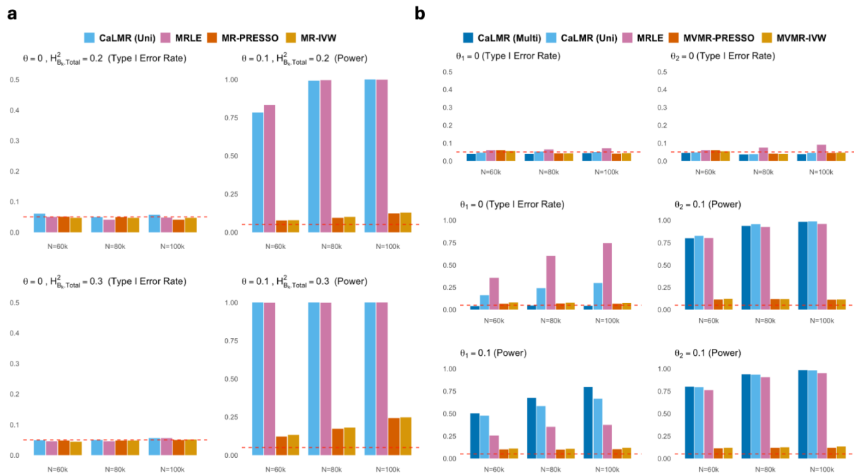
Figure 2: Simulation results under the single-exposure (a) and multiple-exposure (b) scenarios assuming a GWAS sample size for each trait and the outcome N = 60K, 80K, \text{ or } 100K . Results are summarized across 1000 simulations per setting. a. type I error control and power comparison between CaLMR (Uni), MRLE, MR-PRESSO, and MR-IVW under the single exposure setting. The significance threshold for IV selection is equal to p = 5 \times 10^{-4} . We assume the heritability of X is 0.2, and the total heritability of each biomarker H_{B_i, total}^2 = 0.2 (top panel) or 0.3 (bottom panel). b. type I error control and power comparison between CaLMR (Multi), CaLMR (Uni), MRLE, MV MR-PRESSO, and MV MR-IVW in the setting of two correlated latent exposures.
