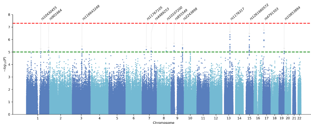
253 Figure 5: Manhattan plot demonstrating the relationship between SNPs and non-responders, 254 highlighting some of the lead SNPs (rsIDs) with pval < 1 x 10 -5 . The green horizontal line at 255 (P = 1E-05) represents the genome-wide significance criterion. Red line represents p-value 256 cut-off of 5E-08.
