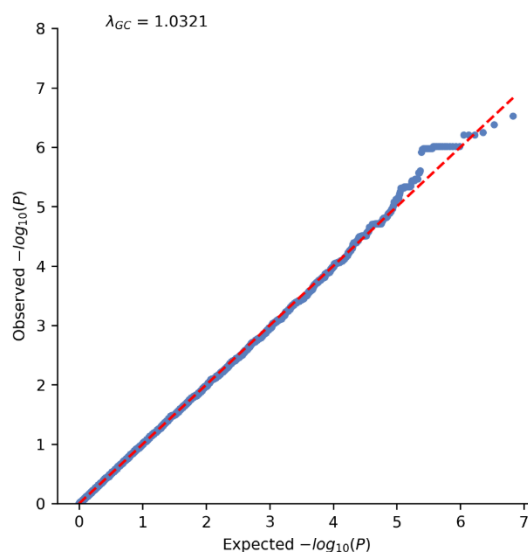
250 Figure 4: QQ (Quantile-Quantile) plot of Non-Responder vs Responder comparison showing 251 the quality of the data with Genomic Inflation rate Estimate: Lambda = 1.0321, representing 252 high-quality data.
