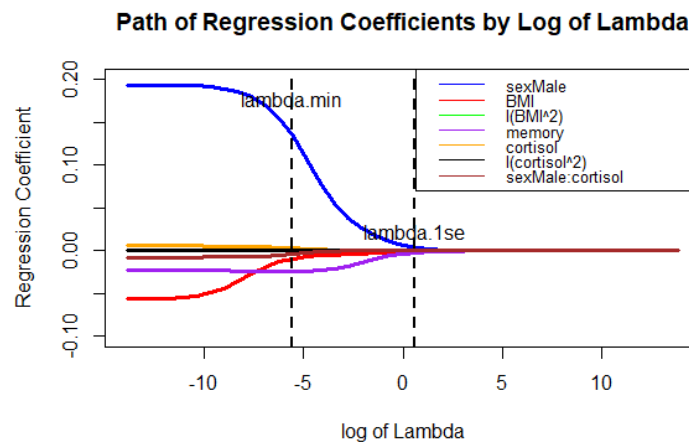
Figure[3]: Ridge regression coefficients change by log of lambda.
