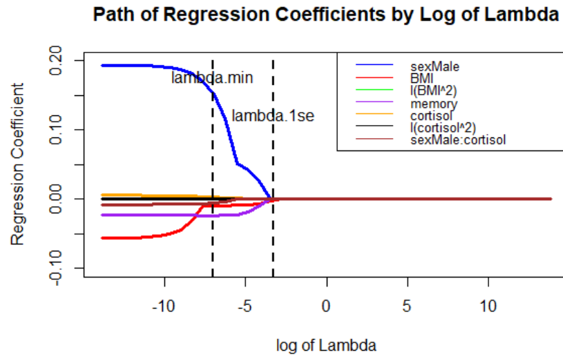
Figure[4]: LASSO regression coefficients change by the log of lambda.
