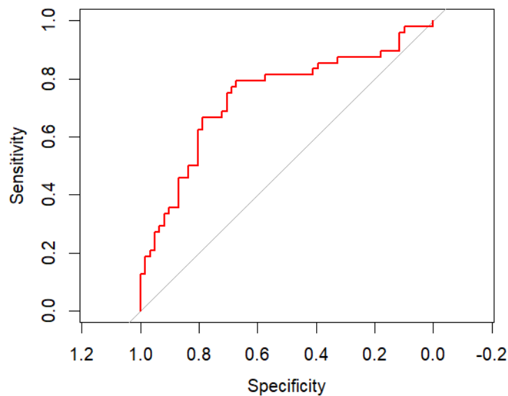
Figure[5]: ROC curve plot of the final logistic model.
