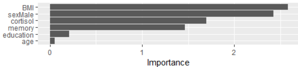
Figure[1]: Variable importance plot (VIP) of all covariates.
