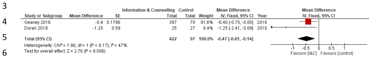
1 Figure 5. Forest plot showing effect of information and counselling measures on salt intake (g/day) 2 in medium term (6 to <12 months)
