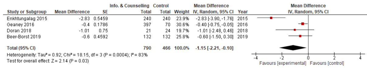
1 Figure 10. Forest plot showing effect of information and counselling measures given at workplaces 2 on salt intake
