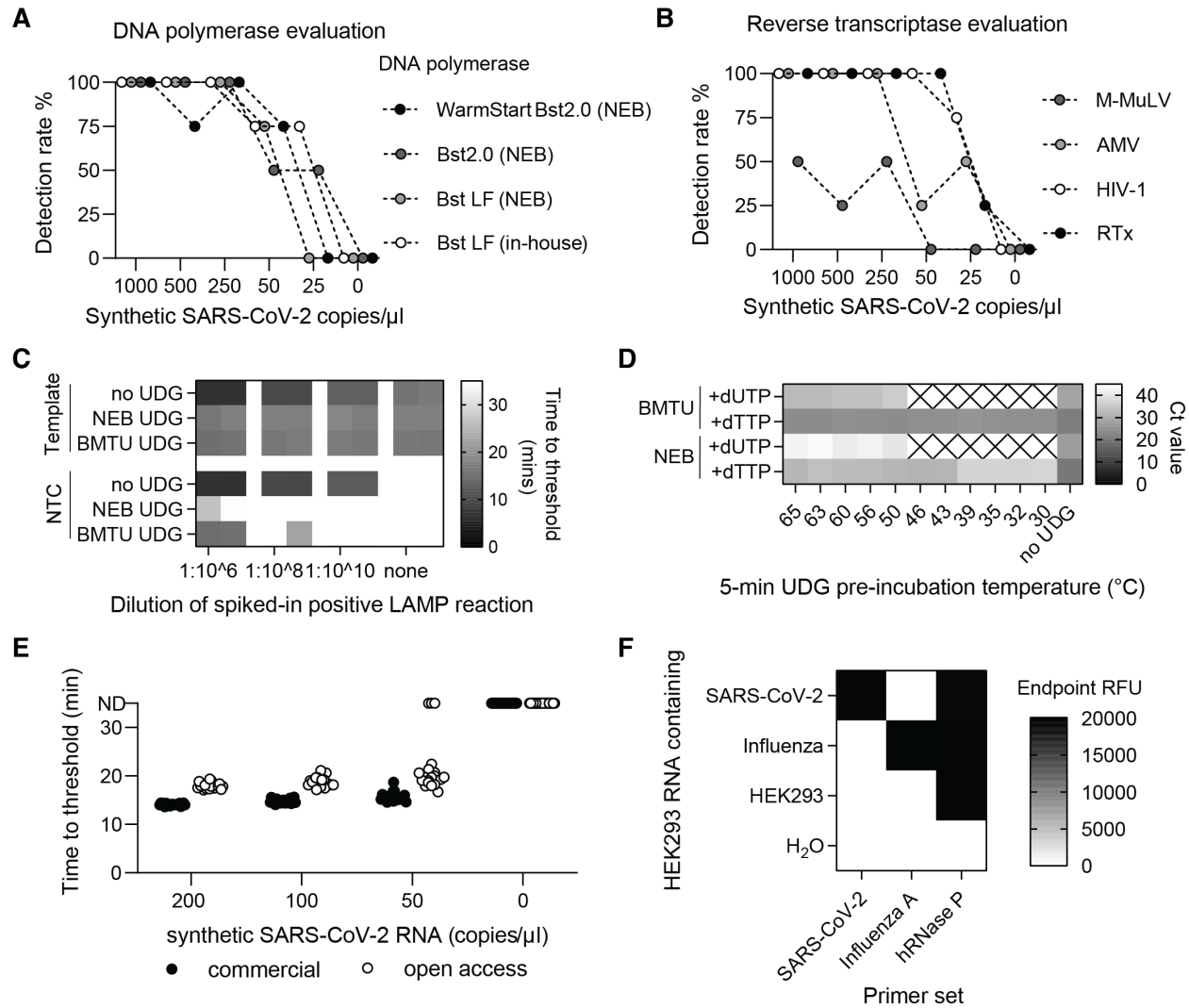
Figure 1: Assessing the performance of open-source RT-LAMP enzymes
