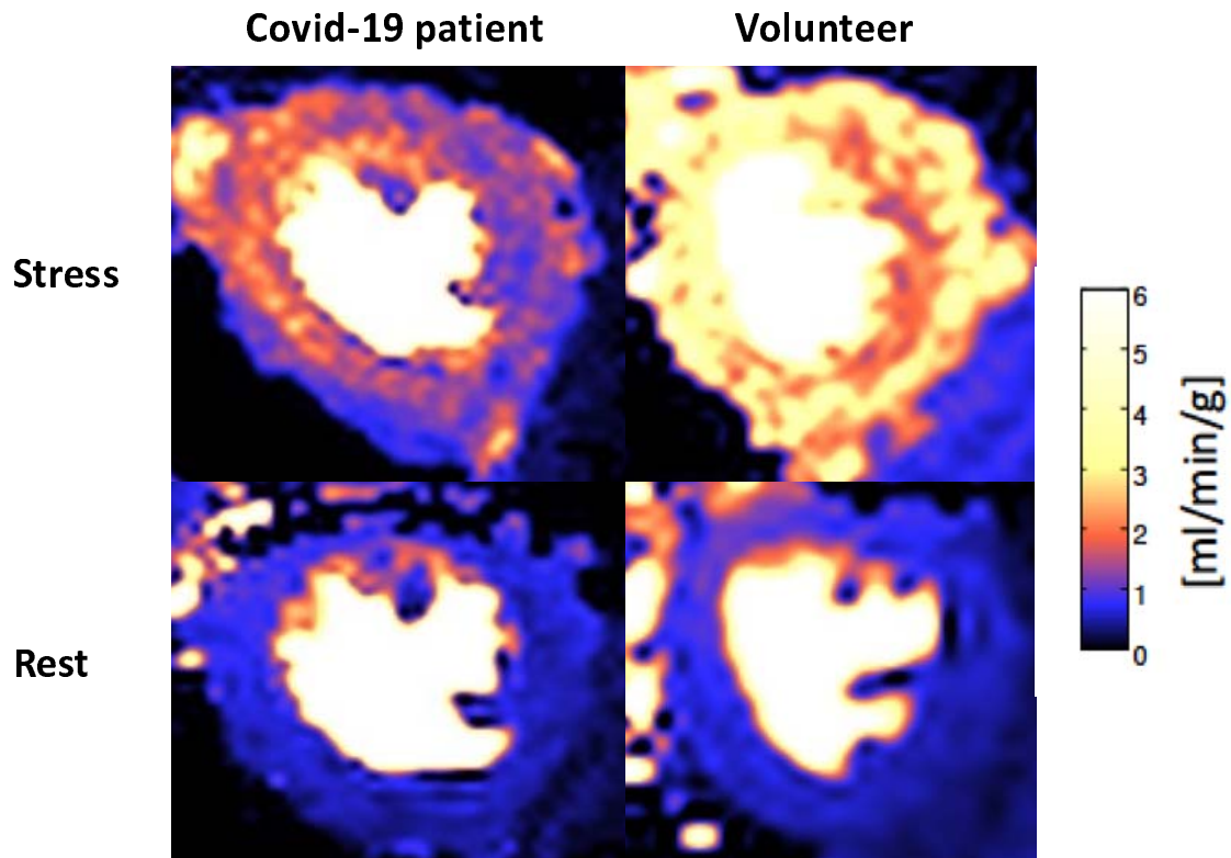
Figure 2. Midventricular perfusion maps of a Covid-19 patient (left) with suspected microvascular dysfunction and a volunteer (right), in stress (upper) and rest (lower). Rest perfusion is comparable, while stress perfusion is globally reduced in the Covid-19 patient compared to the volunteer.
