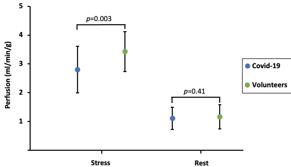
Figure 1. Stress and rest perfusion in Covid-19 patients and volunteers. The figure shows mean and standard deviation together with p-values. Covid-19 patients have lower stress perfusion but comparable rest perfusion, compared to volunteers.
