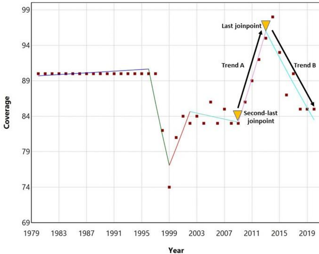
Figure 1. Sample graph displaying the last and second-last joinpoints, as well as trend A-B
