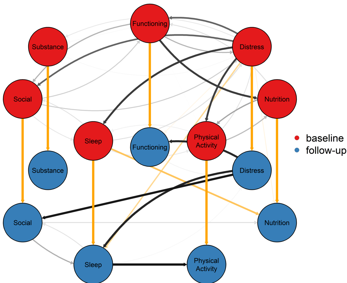
Fig. 2| Consensus graph summarising the posterior distribution of DAGs. Edges between nodes with p_{\text{parent}}>10\% , with darker colours corresponding to higher probability. Yellow arrows show lagged edges whereas grey arrows show within timepoint edges.
