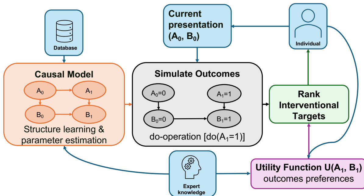
Fig. 1| Causal artificial intelligence recommendation system (CAIRS). CAIRS uses expert knowledge and observational data to learn a causal model, which is then used to simulate outcomes under idealised interventions and displays intervention targets based on their expected utility.
