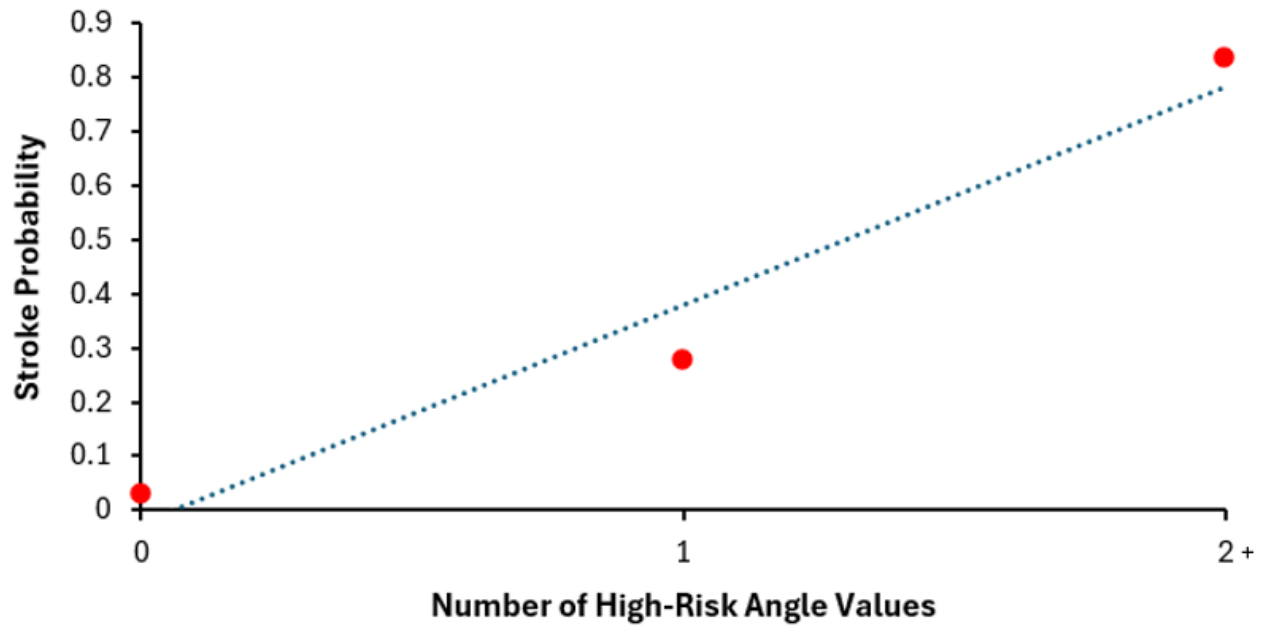
Figure 2. Stroke probability by the number of above-threshold angle values.
