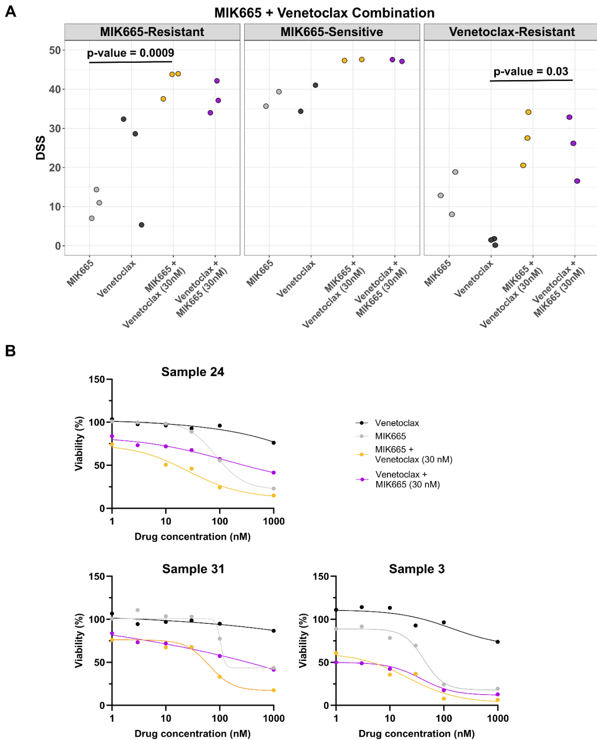
749 Figure 5. A combination of MIK665 and BCL-2 inhibitor venetoclax is more 750 effective compared to each agent alone in selected AML samples.
