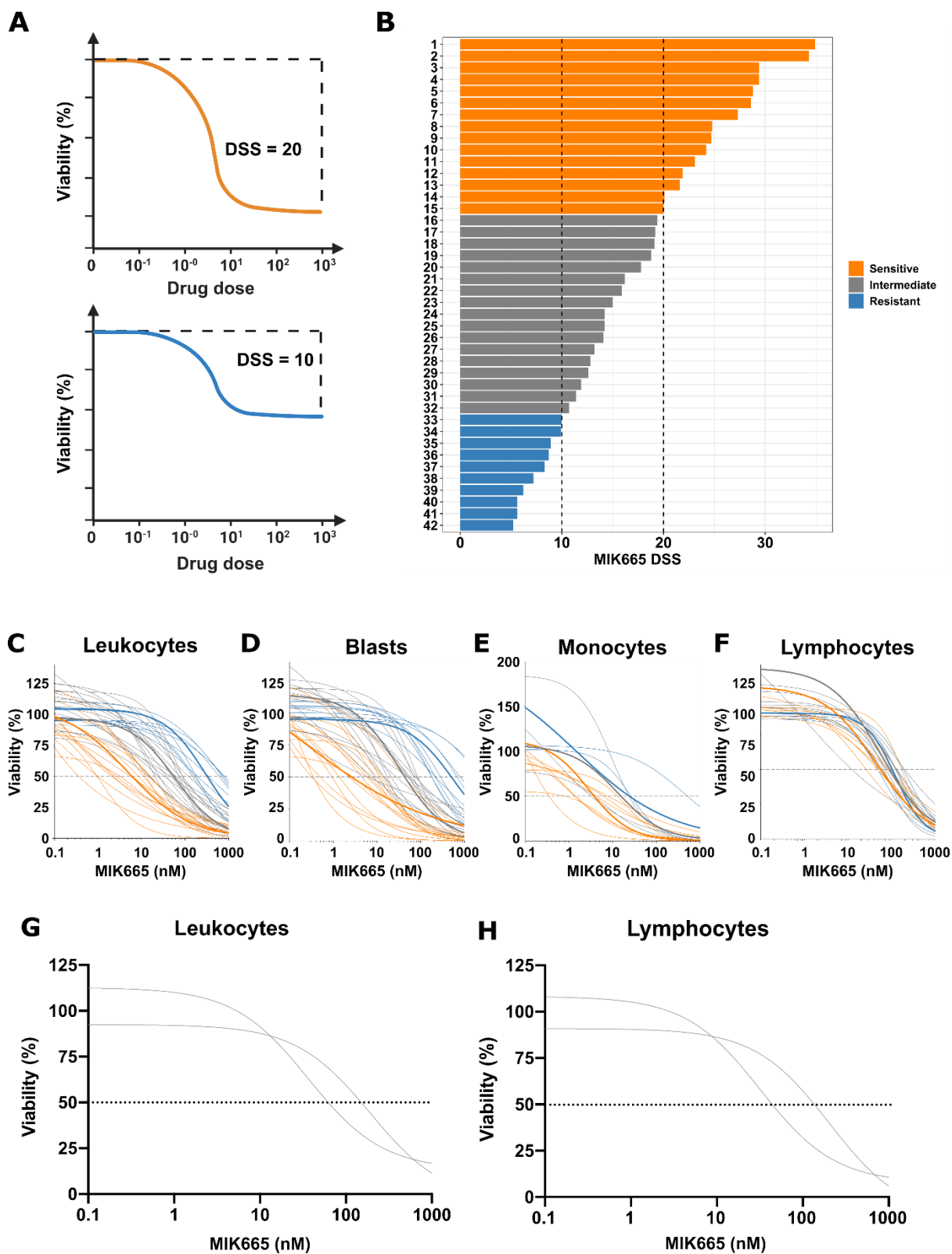
736 Figure 1. Response of AML bone marrow cell populations to MCL-1 inhibitor 737 MIK665.
