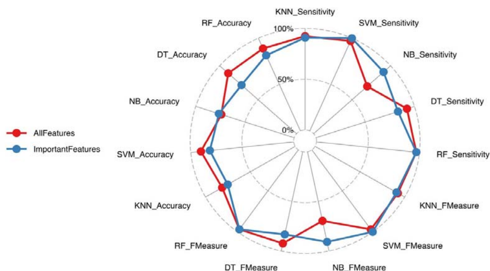
Figure 3- Radar plots depicting the performance of the various algorithms before and after important feature selection for predicting outcomes after Alteplase therapy in ischemic stroke patients.
