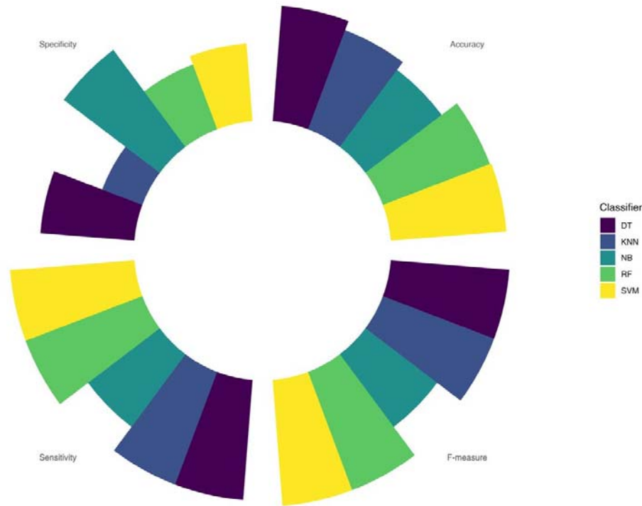
Figure 1: Comparison of F-measure, sensitivity, specificity, and accuracy metrics between KNN, SVM, DT, and RF ML models for predicting outcomes after Alteplase therapy in ischemic stroke patients.
