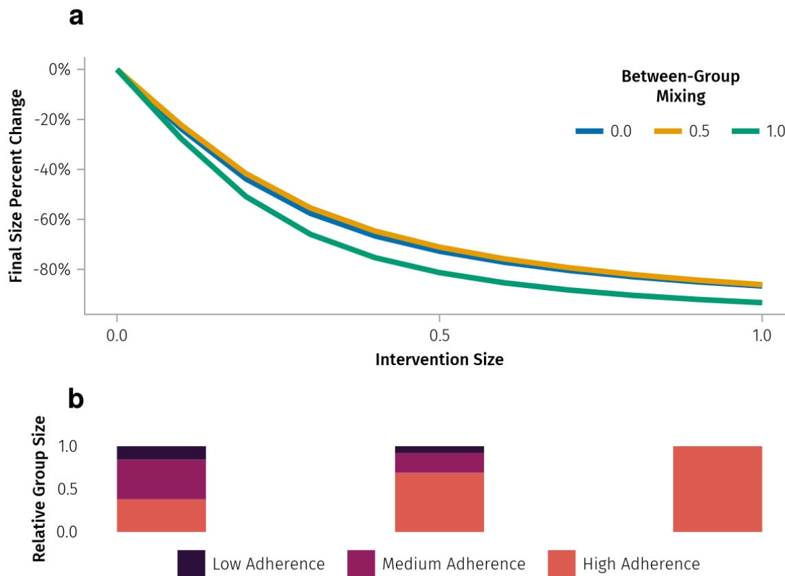
Figure 2: A) The reduction in final infection size across a range of intervention effectiveness (1.0 is a fully effective intervention), accounting for a range of assortativity. Between-group mixing of 1.0 equates to between-group mixing as likely as within-group mixing; B) The relative distribution of group sizes at three levels of intervention effectiveness (0.0, 0.5, 1.0)
