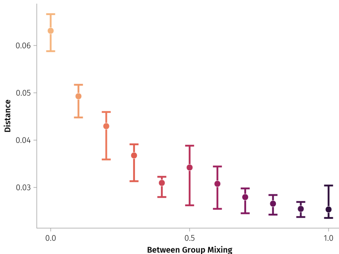
Figure 1: Distribution of the distance from the ABC fits, with the minimum and maximum distances illustrated by the whiskers, and the median distance by the point. Between-group mixing of 1.0 equates to between-group mixing as likely as within-group mixing
