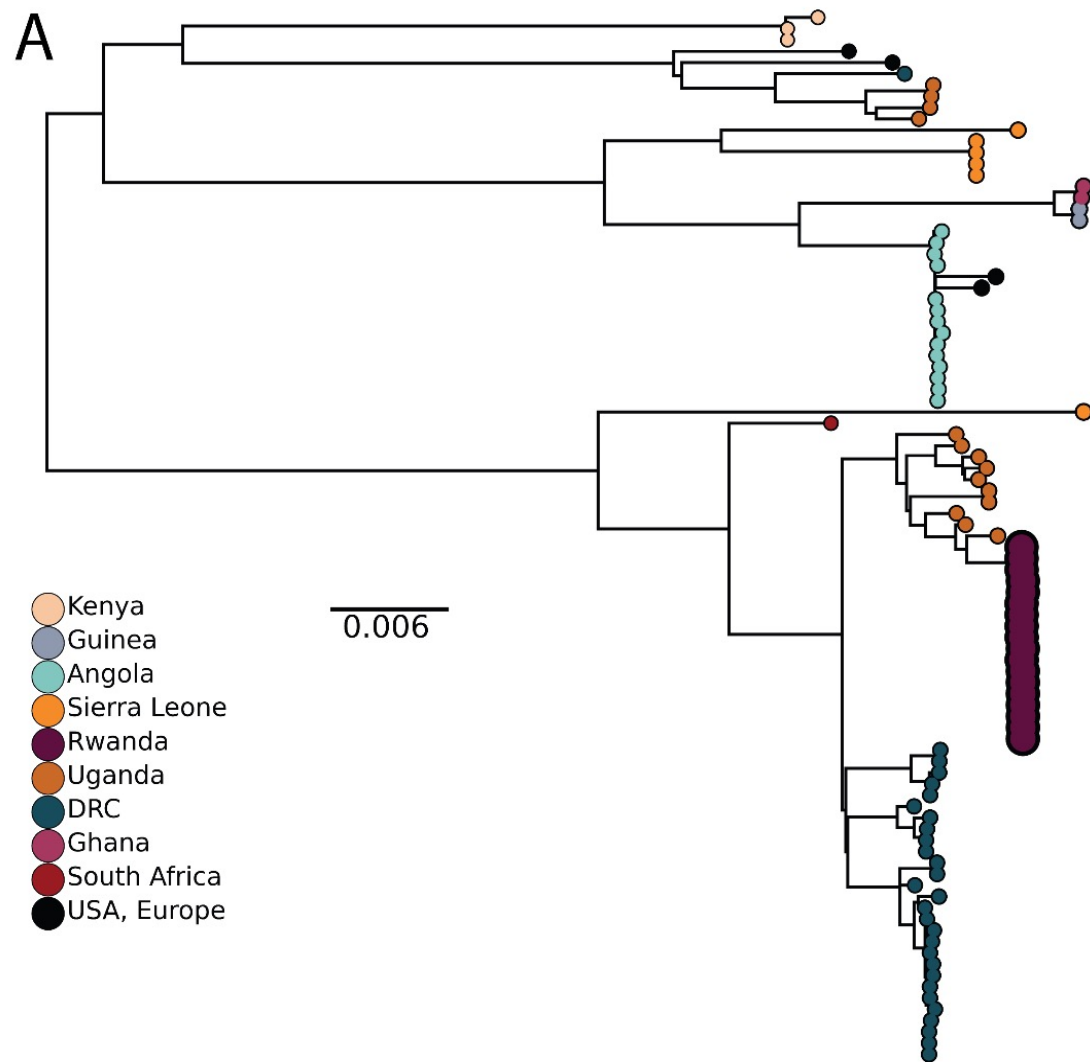
Figure 1: A) Maximum likelihood phylogeny of the global MARV dataset. Tips are annotated by country of isolation. This study's tips are relatively enlarged. B) Map of Uganda and Rwanda. The city of patients in this study (Kigali) is annotated in red. Python Cave and Kitaka Mine in Ibanda district in southwest Uganda are annotated in light blue and yellow, respectively.
