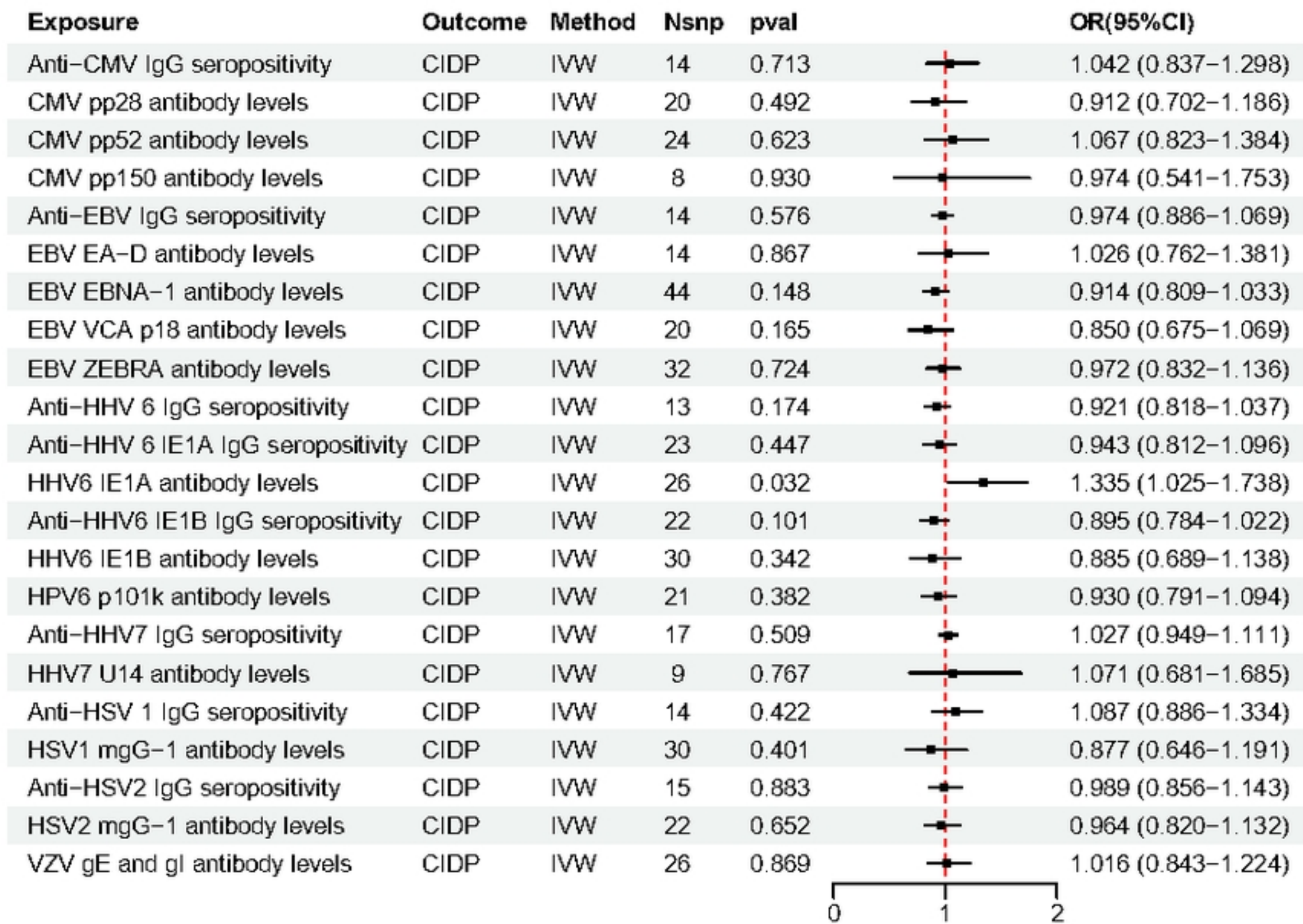
Fig 5 MR estimate results of antibodies of five herpesviridae viru
