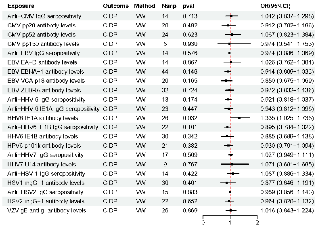
348 Fig 5 MR estimate results of antibodies of five herpesviridae viruses on CIDP.
