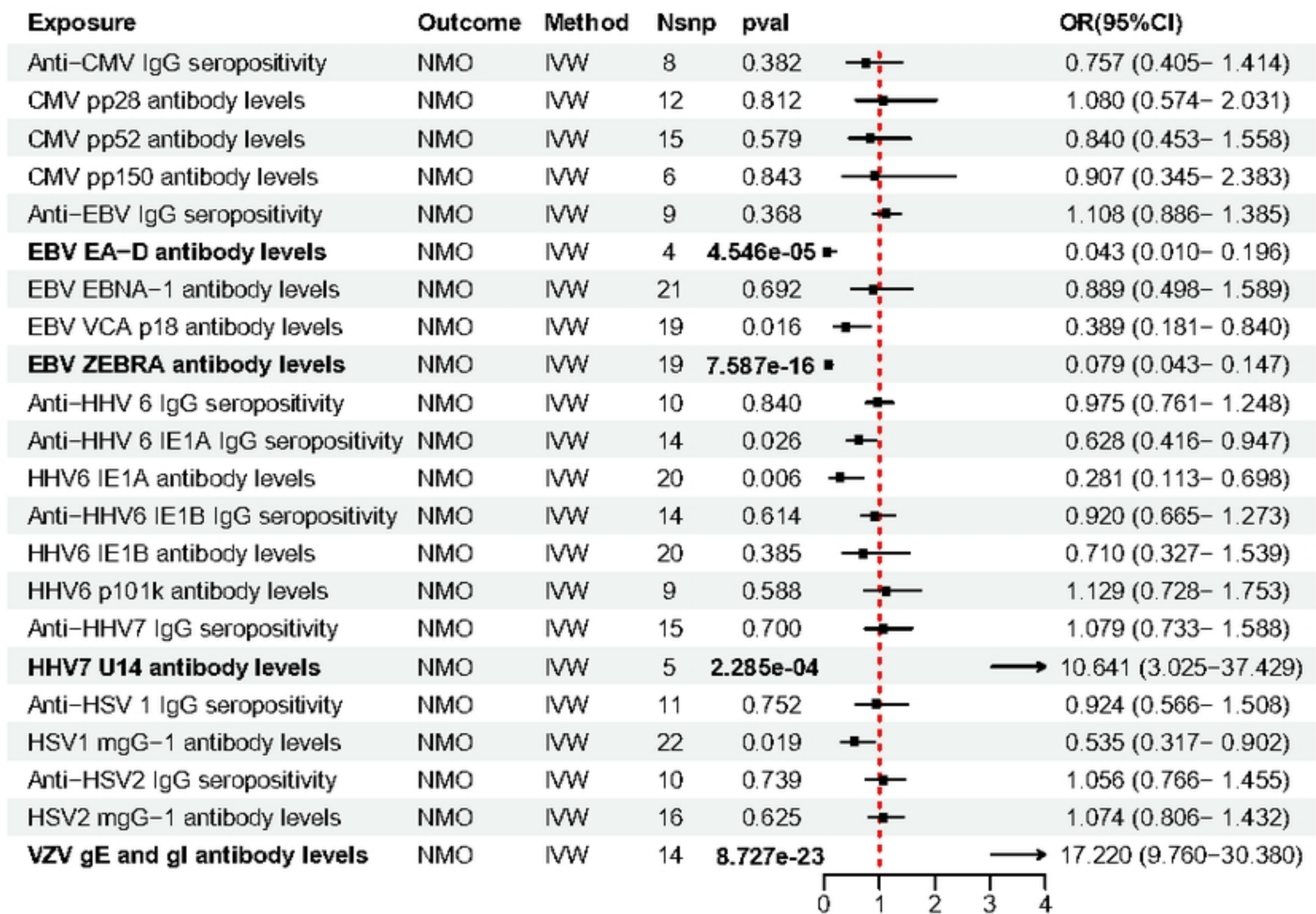
Fig 2 MR estimate results of antibodies of five herpesviridae virus
