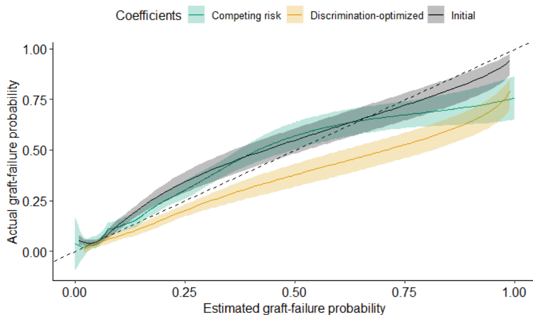
Figure 3: Flexible calibration curve for each possible Kidney Transplant Failure Score. Filled areas show the 95% confidence interval.
