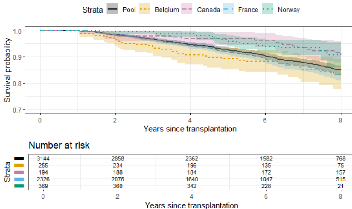
Figure 2: Survival curves for each country and for the pooled validation samples. Notes: The survival probability axis is trimmed before 70% to enhance between-country visibility. The sample is selected among the survivors at one year, i.e., the time of the kidney transplant failure score computation.
