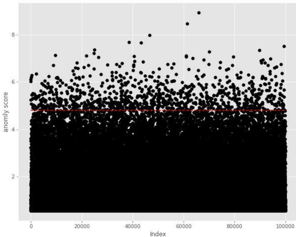
Figure 2 Anomaly detection based on gamma distribution in CNN model, showing the distribution of the anomaly scores for the predicted possibility in the test data. Anomaly score was calculated as the minus logarithm of the probability density in the gamma distribution for each sample in the test data. The red dashed line is the threshold, using an anomaly score of 4.8, above which the sample was considered abnormal.
