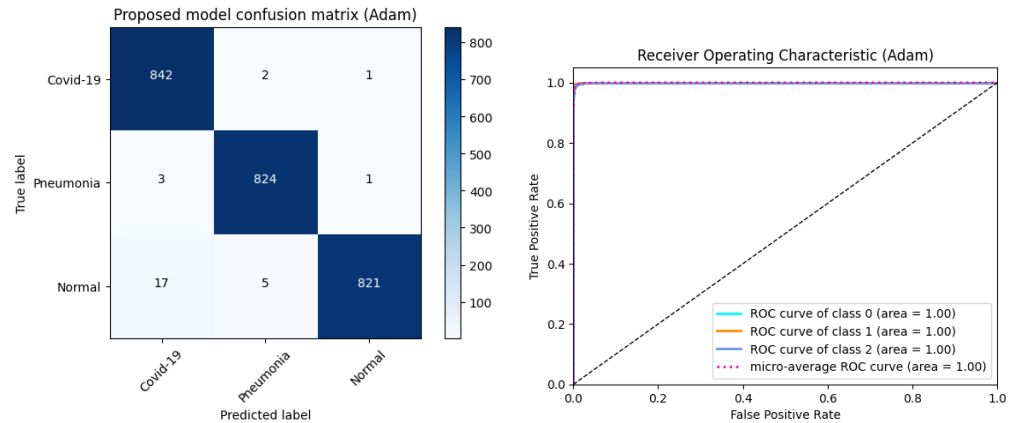
Fig 9. Proposed model confusion matrix for X-ray Image Dataset
