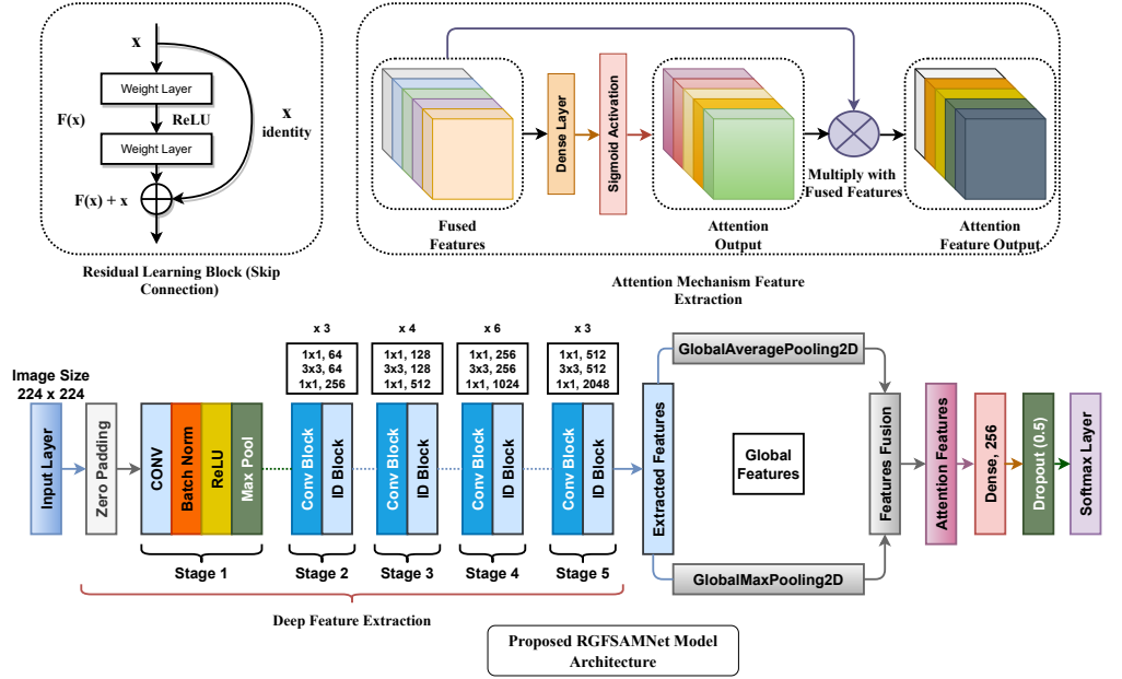
Fig 4. Schematic architecture of the proposed model.
