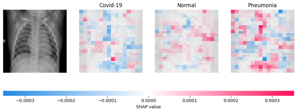
Fig 16. SHAP-based visualization for the proposed model for X-ray image
