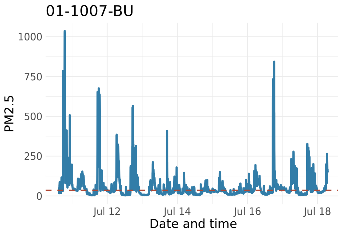
Figure 1b: Color-coded graph using the PM 2.5 standard from WHO for the average PM 2.5 level during the measurement period
