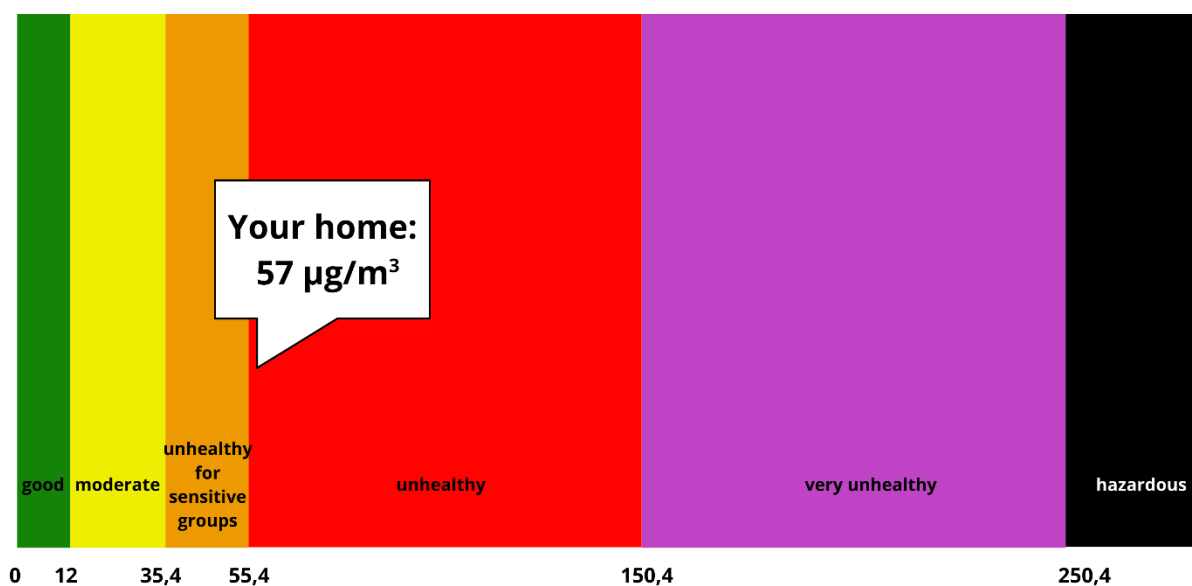
Figure 1b: Color-coded graph using the PM 2.5 standard from WHO for the average PM 2.5 level during the measurement period
