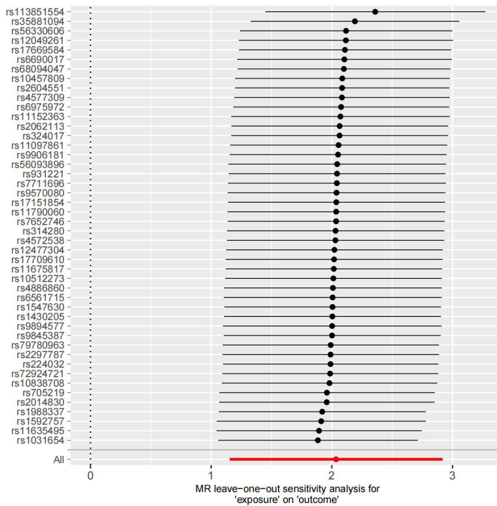
Fig.4 Leave-one-out sensitivity analysis of the effect of FM on insomnia
