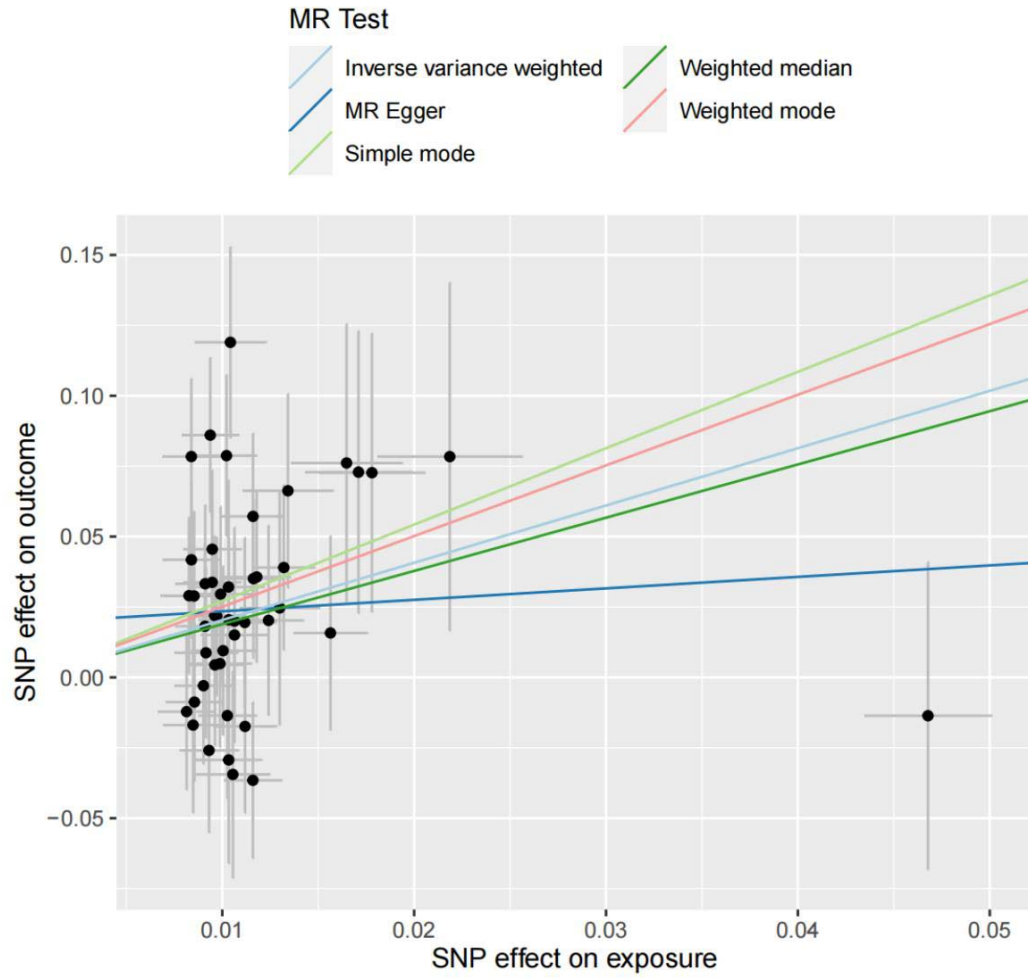
Fig. 1 Scatter plot of the causal effect of insomnia on FM
