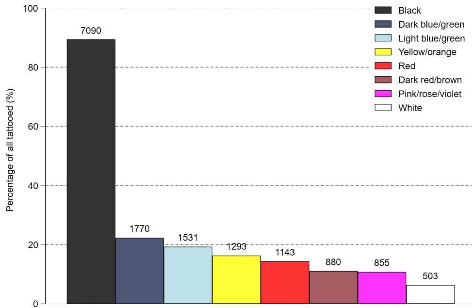
Figure 2: Frequency and percentage of tattoo colours in the tattooed subsample with full exposure information.
