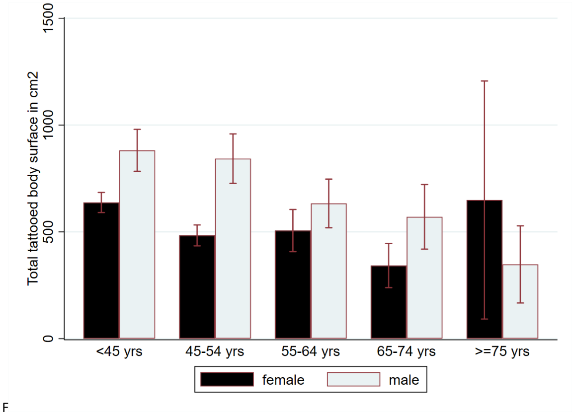
Figure 1: The mean total body surface tattooed by biological sex over age categories in the tattooed subsample with full exposure information.
