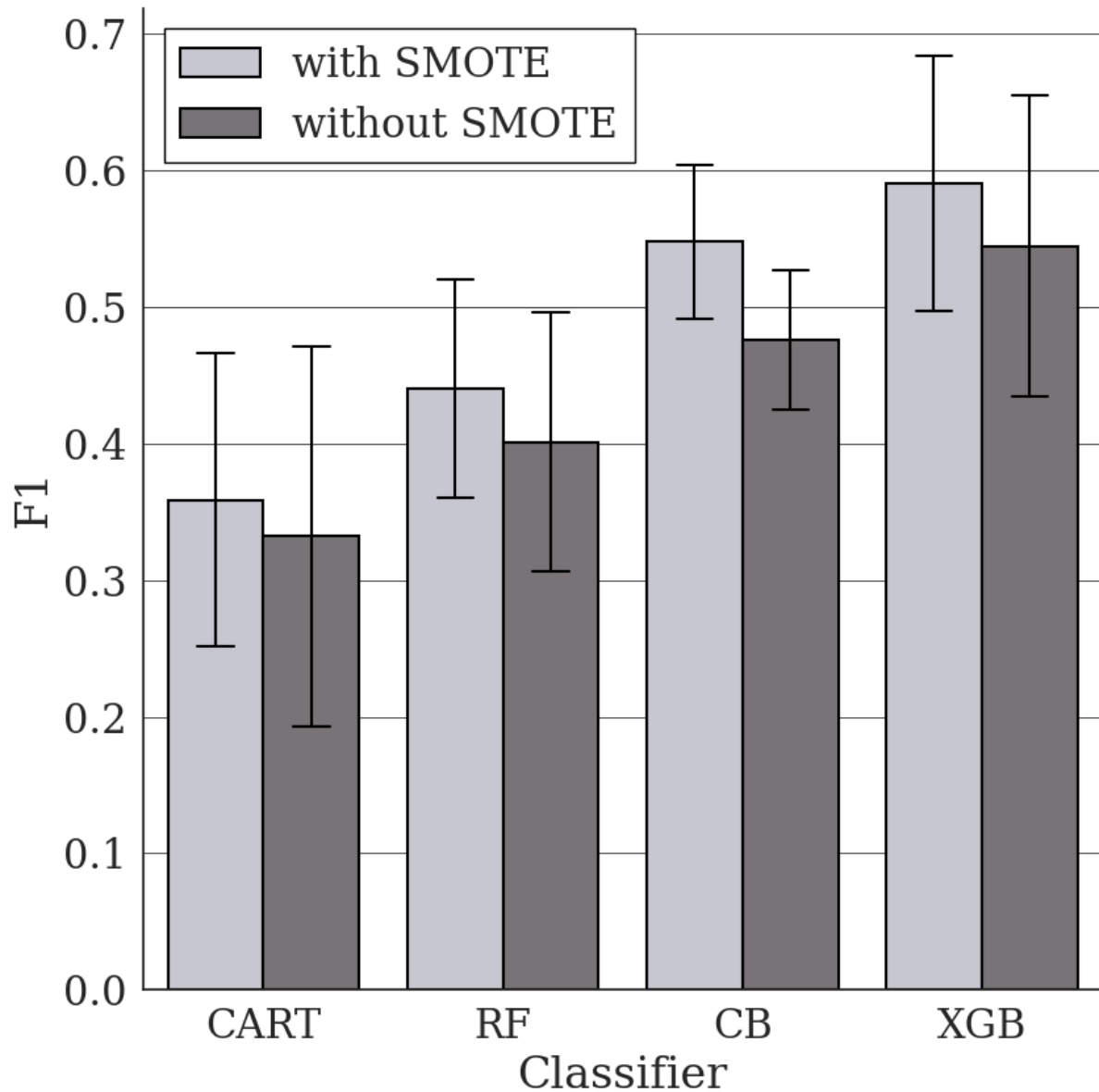
Figure 1: Mean ( \pm SD) F1 score for classifier models on the whole cohort. Models were cross-validated over ten folds containing data from 460 patients. This was repeated twice, once using SMOTE during training to upsample the minority class (those who did develop de novo HLA-specific antibody) to the same size as the majority class, and once without.
