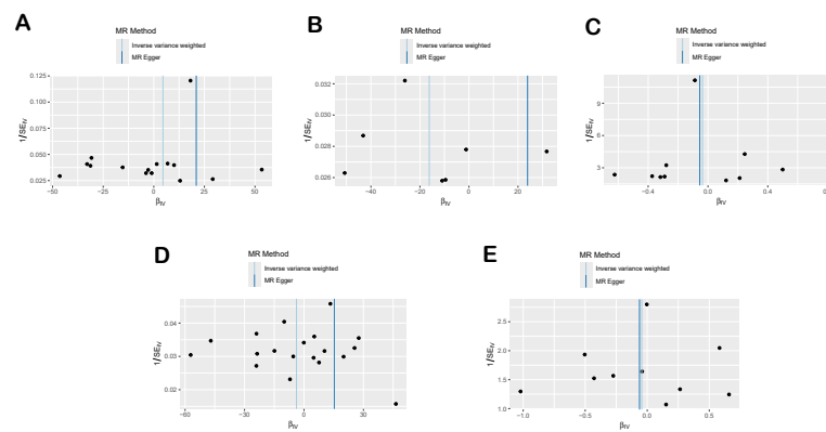
Fig. 5 Funnel Plot
