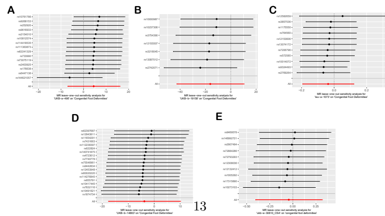
Fig. 4 Leave-One-Out Plot
