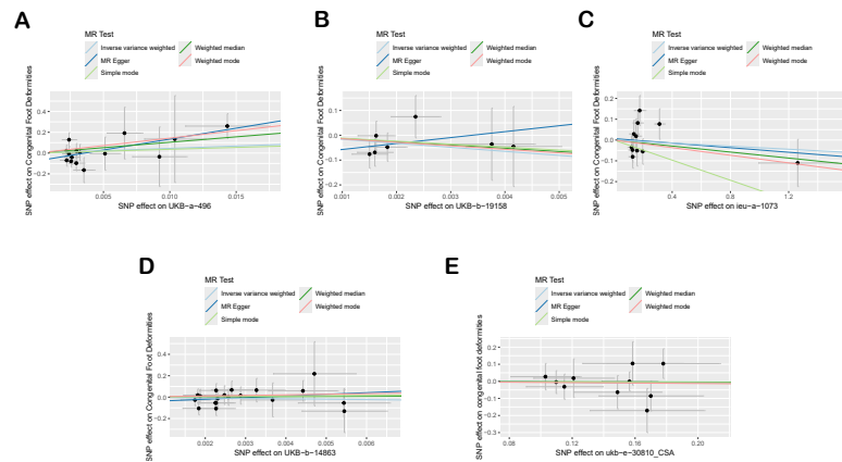
Fig. 2 Scatter Plot
