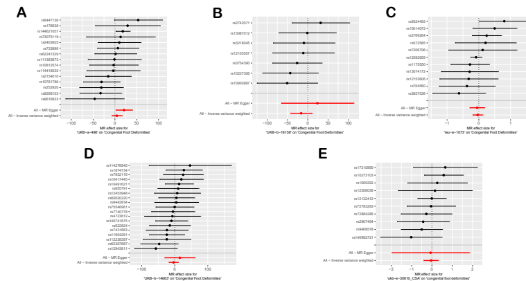
Fig. 3 Forest Plot
