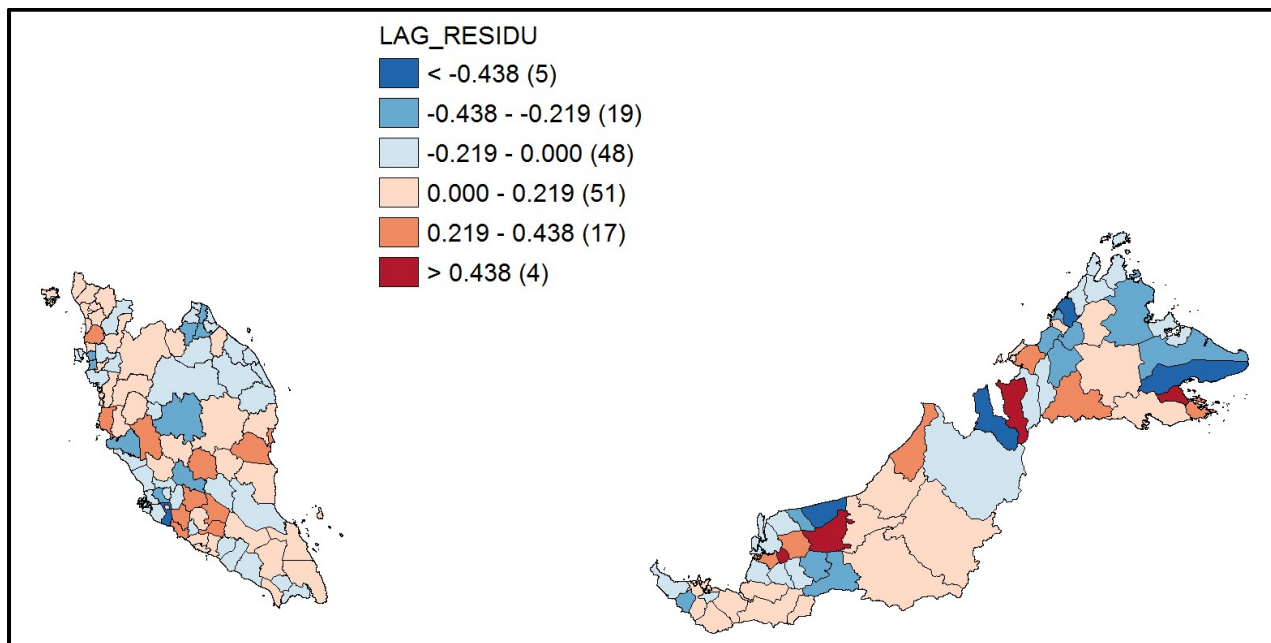
Results showing a standard deviation map of the Spatial Lag Regression (SLM) model residuals by administrative districts in Malaysia.
