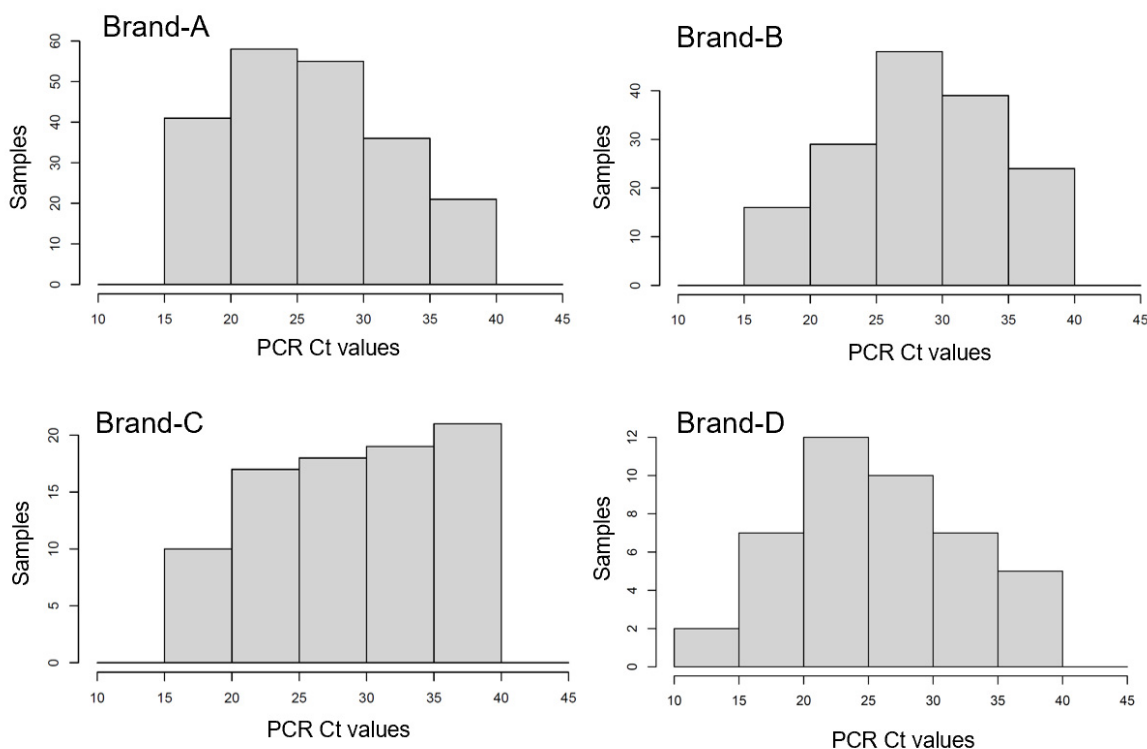
Figure 2. Histograms of the samples qRT-PCR cycle count (Cts) for the four datasets analyzed, each one corresponding to a different AT supplier. The Cts shown are the average between the cycle counts of gene N and gene ORFab.
