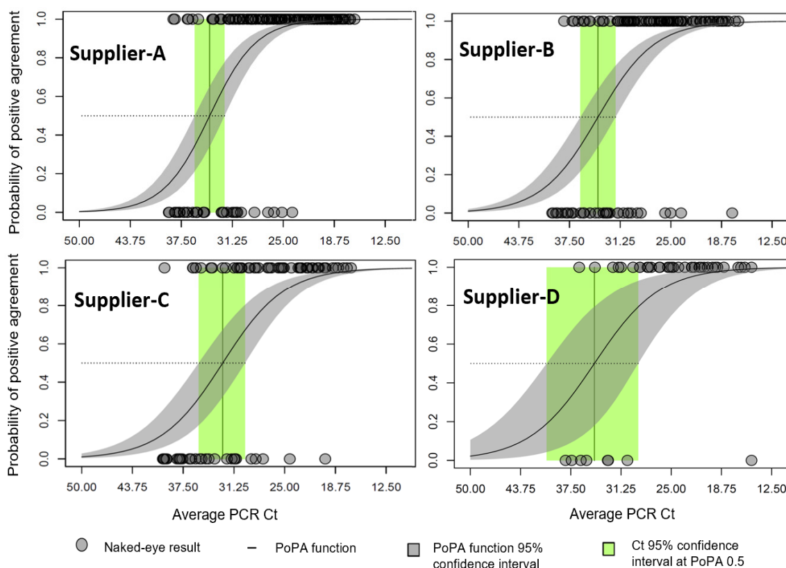
Figure 3. Probability of positive agreement (PPA) as function of the qRT-PCR cycle count (Ct) for naked-eye assessments of the Chelsea project participants after self-application of the antigen tests. Naked-eye assessments of the antigen test result are plotted in the vertical axis with value 1 for positive and 0 for negative. The PPA function is obtained by logistic regression of the binary naked-eye results, and shows the strong dependency of the agreement probability with the qRT-PCR Ct's.
