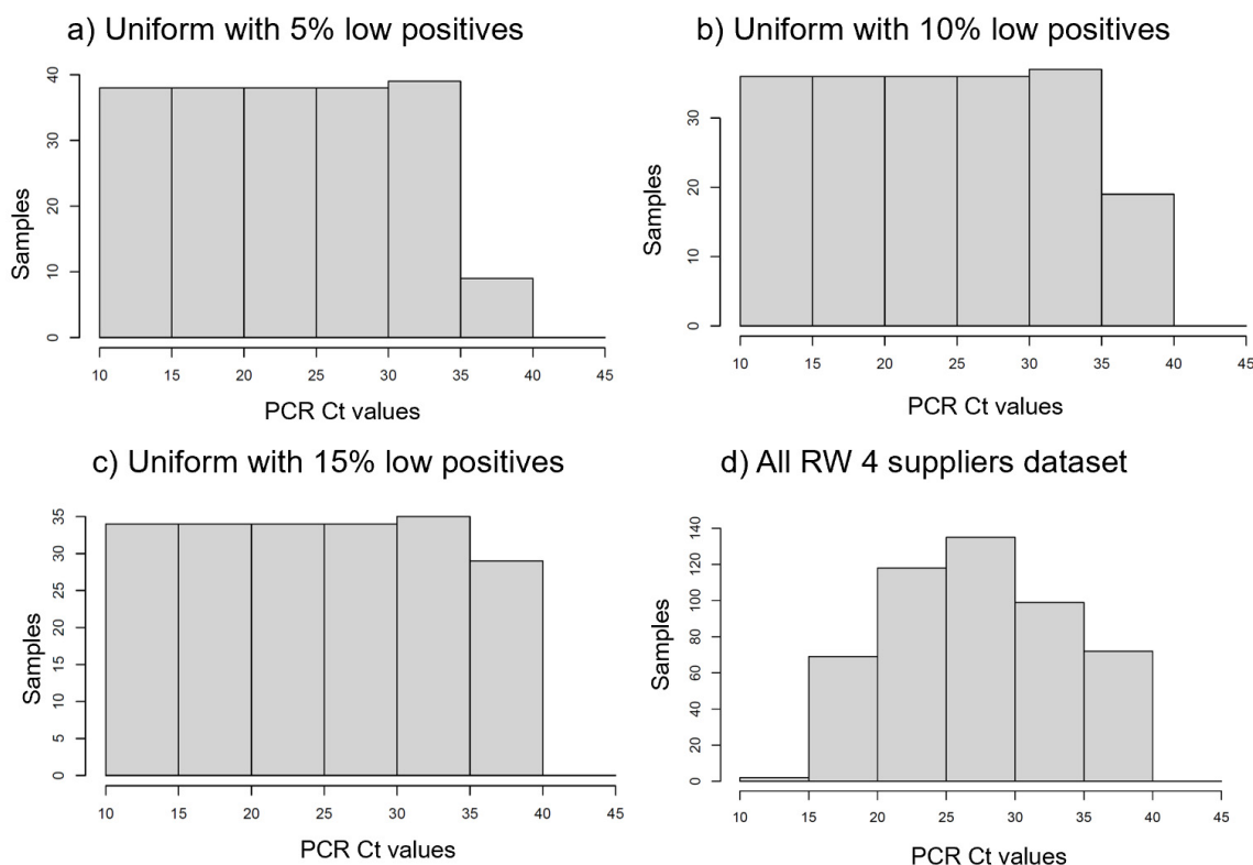
Figure 4. Four different reference distributions used to correct the raw data sensitivity calculations from uneven viral concentration sampling. Histograms a, b, and c correspond to 200 cases with variable fraction of low positives (35-40 Cts) and uniform distribution in the 10-35 Ct range. Histogram d corresponds to the joint four supplier's observed data.
