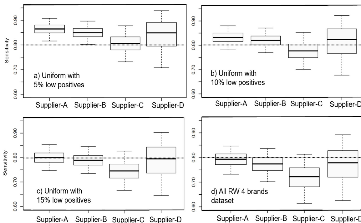
Figure 5. Sensitivity corrected from the uneven distribution of viral concentration across the four supplier's datasets, and corresponding to the four optional referential distributions of qRT-PCR cycles shown in figure 4. The boxes show 50% and the segments 95% confidence limits. The dotted line shows the 0.8 sensitivity threshold.
