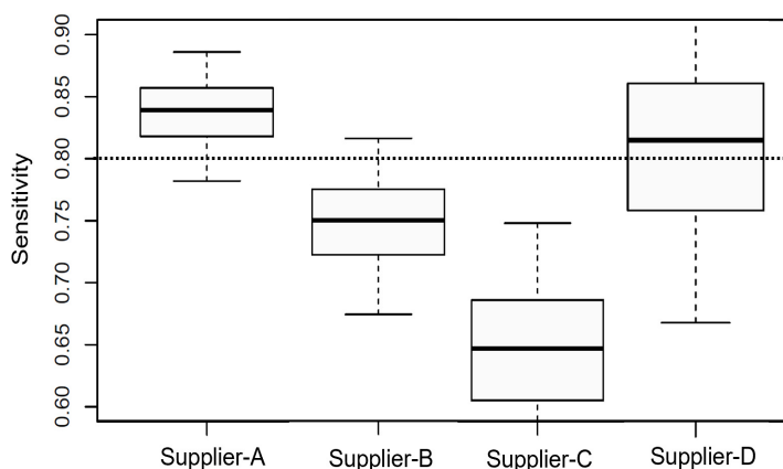
Figure 1. Sensitivities calculated from the raw data from the Chelsea study for suppliers A, B, C and D. The boxes show 50% and the segments 95% confidence limits calculated with the Clopper-Pearson method. The dotted line shows the 0.8 sensitivity shred hold.
