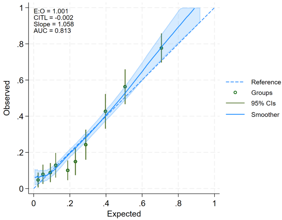
Figure 1. Calibration plot of Lebanese depressive symptom prediction model
