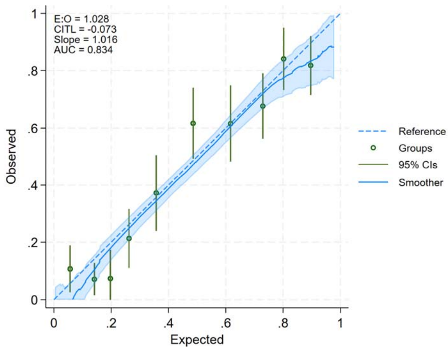
Figure 2. Calibration plot of Syrian depressive symptom prediction model
