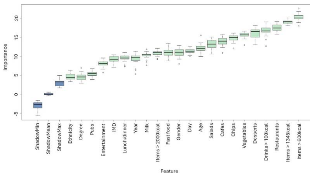
Figure 1: Random Forest Model feature importance with all predictors
