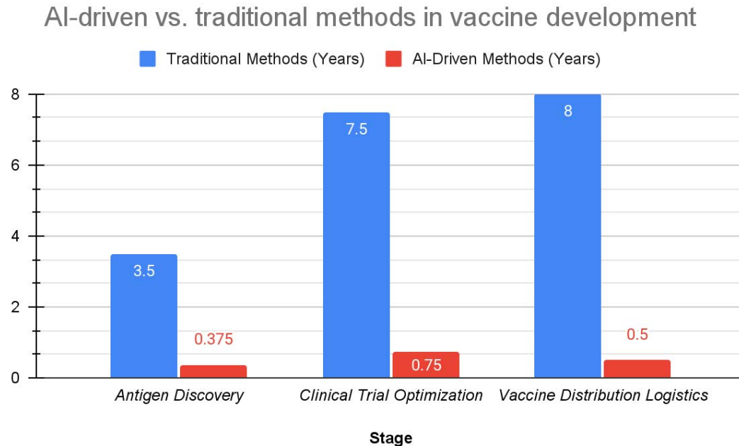
Figure 3: This table summarizes the differences between traditional and AI-driven methods across various stages of vaccine development. It shows how AI models, particularly in antigen discovery and clinical trial design, drastically reduced the time and complexity of these stages compared to traditional methods, cutting years down to months.
