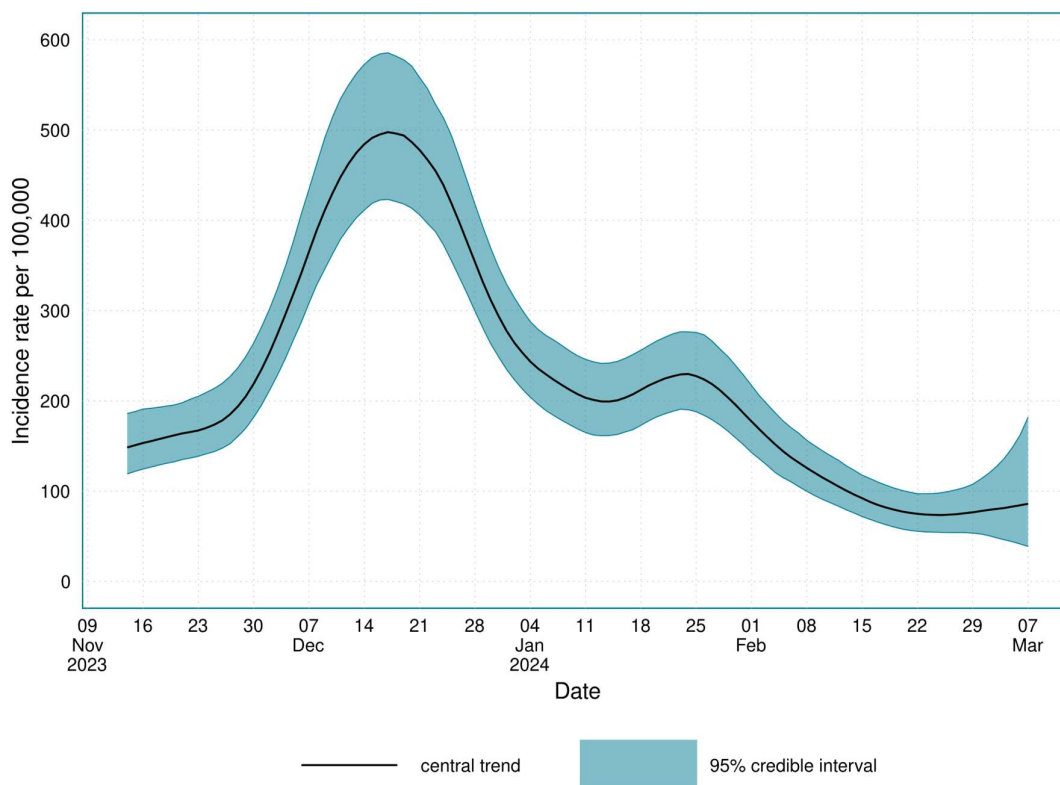
Figure 4: The incidence of SARS-CoV-2 infections in England and Scotland from the 14 th November 2023 to the 7 th March 2024.
