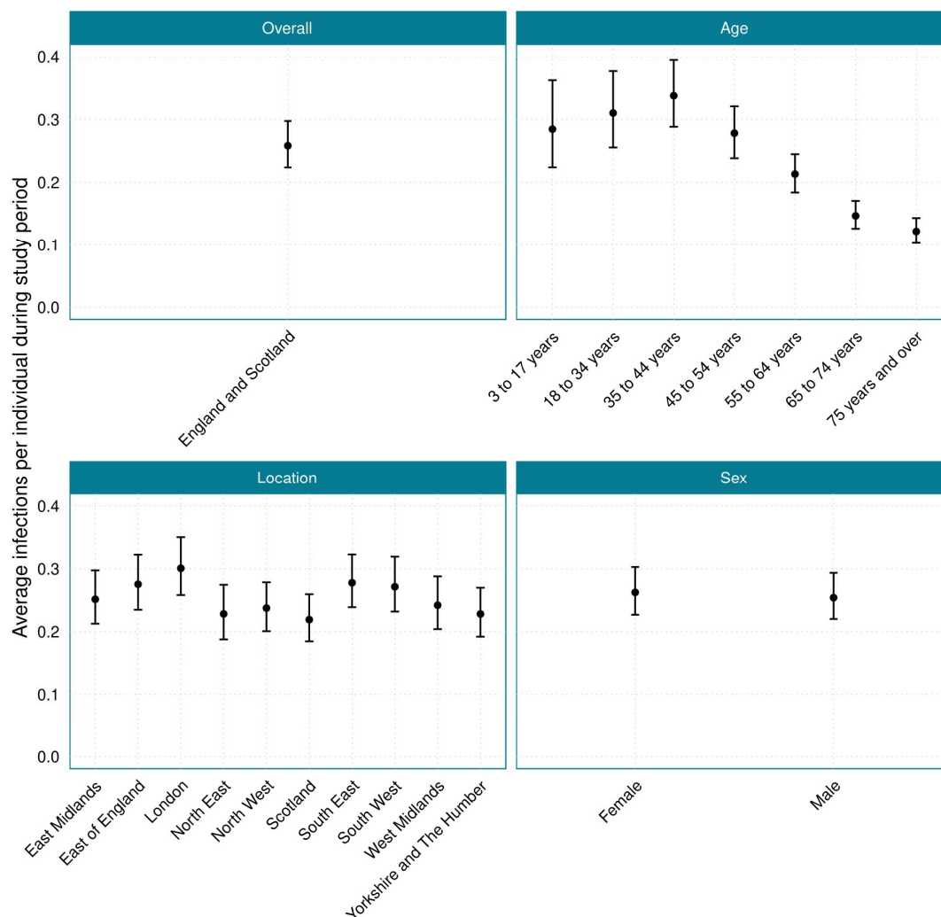
Figure 7: The average number of infections that occurred per individual during the study period, 14 th November 2023 to 7 th March 2024, for England and Scotland and when stratified by age, location, and sex.
