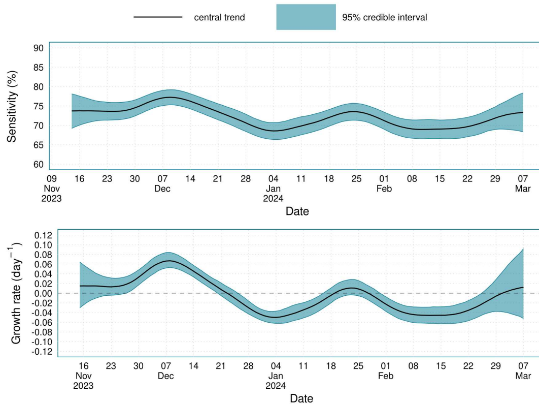
Figure 8: Estimates of average LFD sensitivity and the incidence exponential growth rate for England and Scotland from the 14 th November 2023 to the 7 th March 2024.
