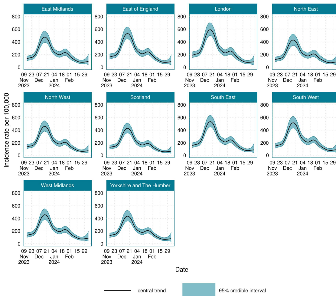
Figure 6: The location-stratified incidence of SARS-CoV-2 infections in England and Scotland from the 14 th November 2023 to the 7 th March 2024.
