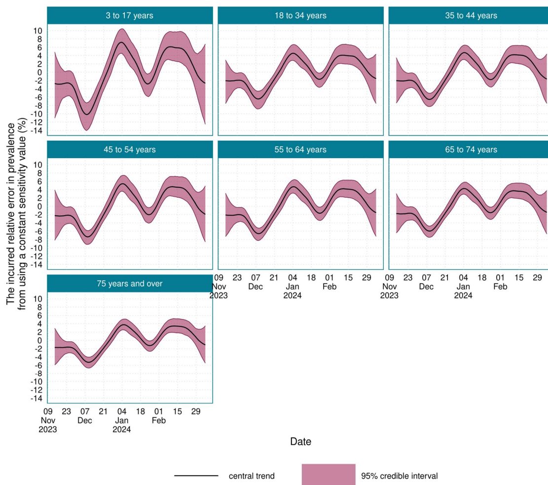
Figure 10: The relative error in the prevalence estimate, Error_{a,s,l}(t) , that is incurred from using a constant value of LFD test sensitivity, rather than the time-varying value of LFD test sensitivity that was estimated by the model.
