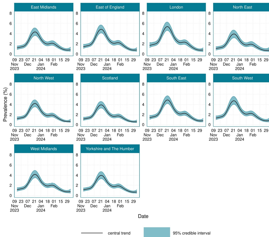
Figure 3: The location-stratified prevalence of SARS-CoV-2 in England and Scotland between the 14 th November 2023 and the 7 th March 2024.
