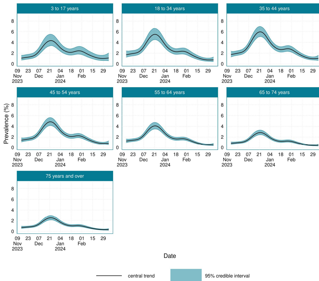
Figure 2: The age-stratified prevalence of SARS-CoV-2 in England and Scotland between the 14 th November 2023 and the 7 th March 2024.
