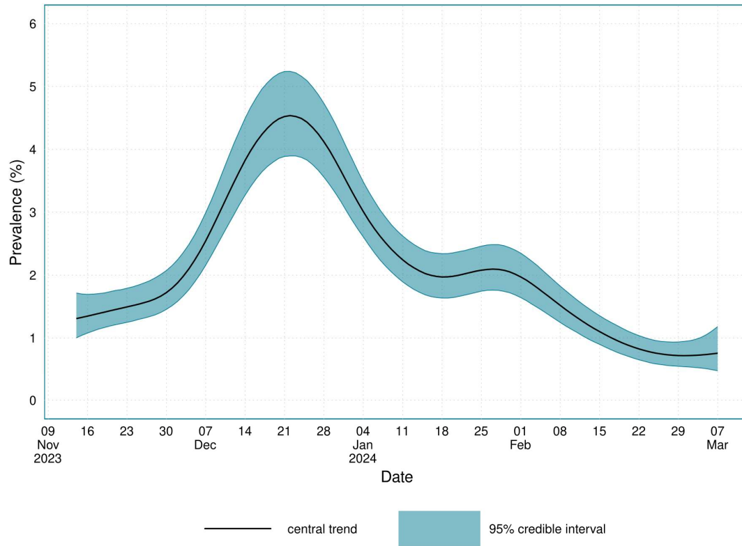
Figure 1: The prevalence of SARS-CoV-2 in England and Scotland between the 14 th November 2023 and the 7 th March 2024.
