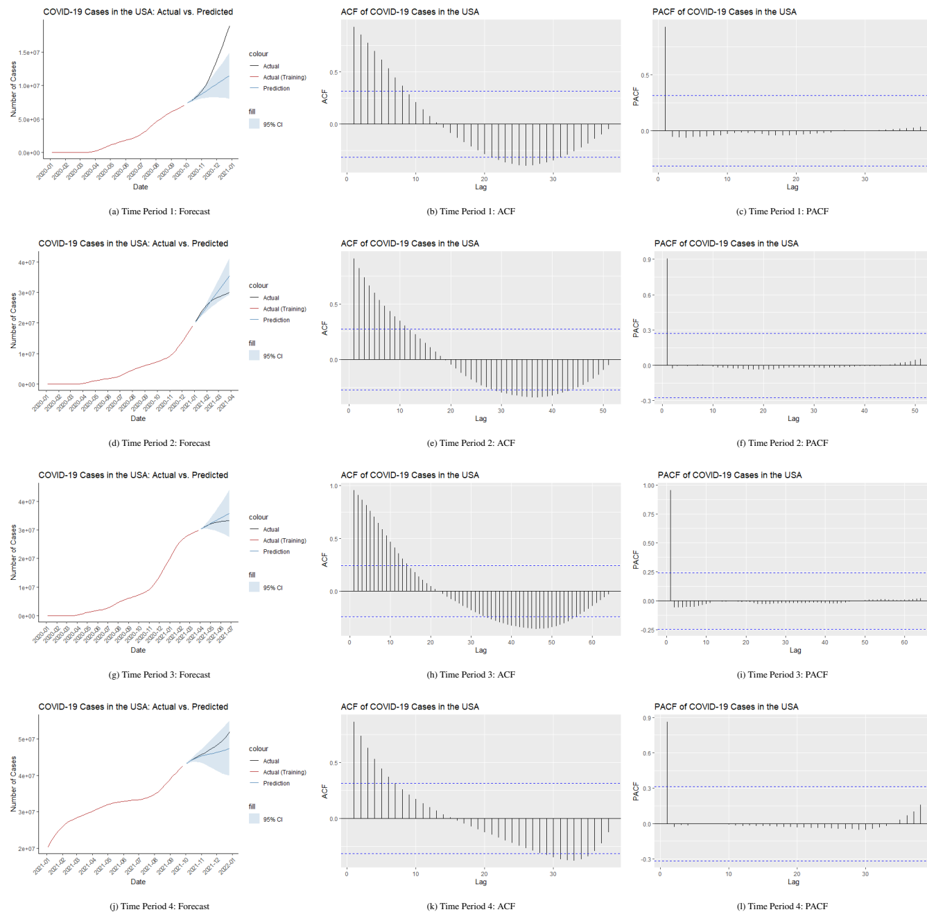
FIGURE 2 ARIMA Model Analysis in the U.S. Over Different Time Periods
