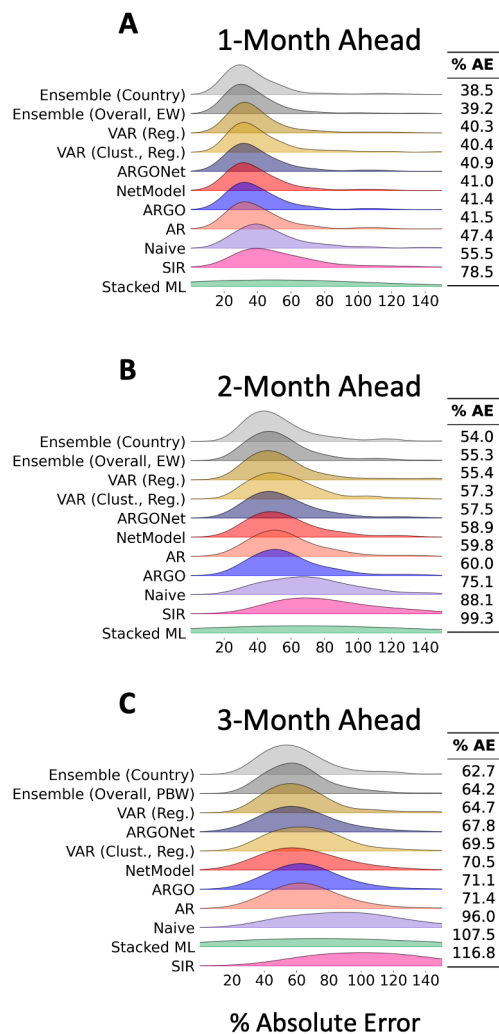
Figure 3: Overall error distributions for optimized individual and ensemble models across all 187 tested locations. (A) - (C) Ridgeline plots show percent absolute error distributions at the 1-month, 2-month, and 3-month horizons, respectively. Side tables record the mean percent absolute error incurred.
