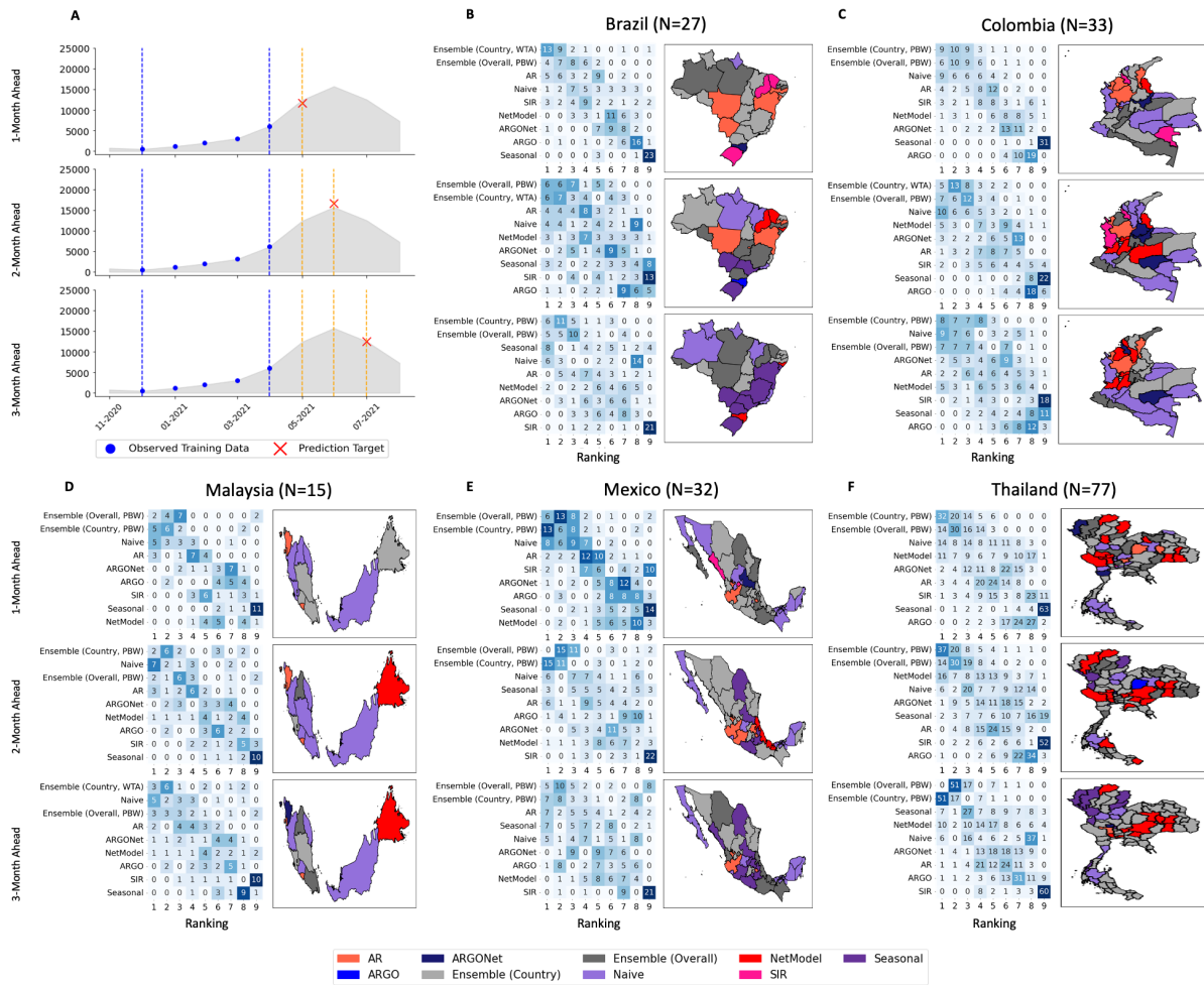
Figure 11: Country-specific standard individual and ensemble model performance rankings. (A) Graphical representations of the 1-, 2-, and 3-month forecast horizons. The red X marks our forecasting target n -months ahead, the blue dots represent the historical cases that we are using as our observed training data (in this case, a 5-month window), the vertical blue dotted lines represent the limits of our training data range. The grey silhouette represents the ground truth reported case counts. (B) - (F) Within each country and forecast horizon, the heatmaps show the rankings distribution for each individual and ensemble model's forecasts in terms of percent absolute error. The geographic maps next to each heatmap indicate the best-performing model in each province, color-coded by the legend at the bottom of the figure.
