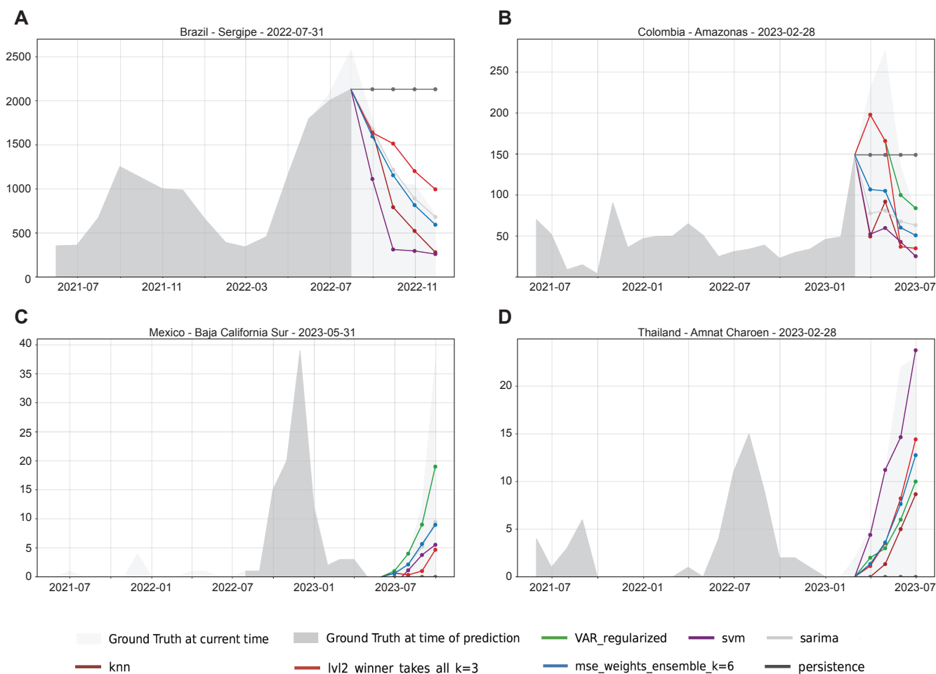
Figure 7: Visualization of the bias embedded in our models given reporting delays. The official reports known at the time of prediction, shown in dark gray, is the only information available to our models at the time of prediction. After several months, the ground truth changes due to backfill efforts based on the most recent reports are shown in light gray.
