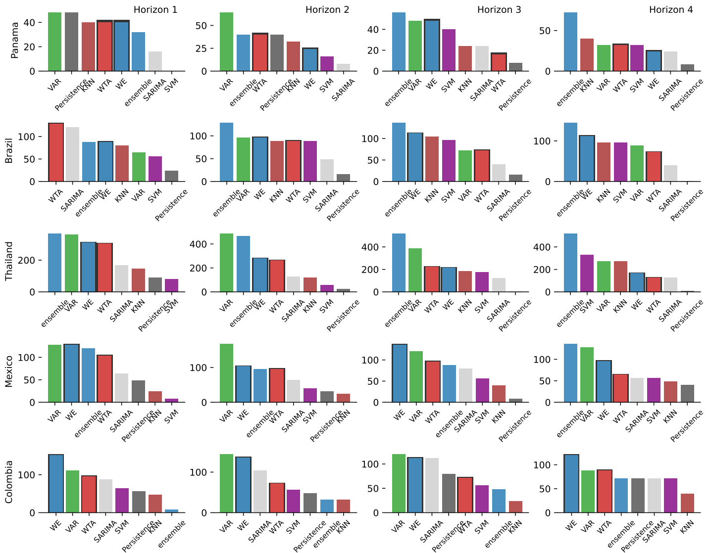
Figure 5: Top performer count. A visualization of the number of times a model scored a value of MSE rated among the top 3 best, ordered from left (models with the highest count) to right (models with the lowest count). Our results show that the Weighted Ensemble (blue), VAR (green), and the Winner-Takes-All approach are frequently among the top performers (leftmost side).
