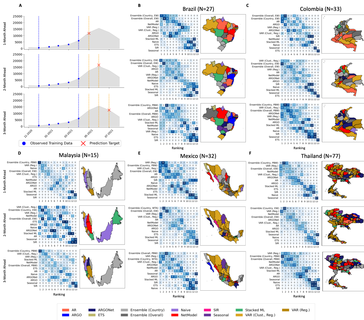
Figure 1: Country-specific optimized individual and ensemble model performance rankings. (A) Graphical representations of the 1-, 2-, and 3-month forecast horizons that we explore in this paper. The red X marks our forecasting target n -months ahead, the blue dots represent the historical cases that we are using as our observed training data (in this case, a 5-month sliding window), the vertical blue dotted lines represent the limits of our training data range, and the grey silhouette represents the ground truth reported case counts. (B) - (F) Within each country and forecast horizon, the heatmaps show the rankings distribution for each individual and ensemble model's forecasts in terms of percent absolute error. The geographic maps next to each heatmap indicate the best-performing model in each province, color-coded by the legend at the bottom of the figure.
