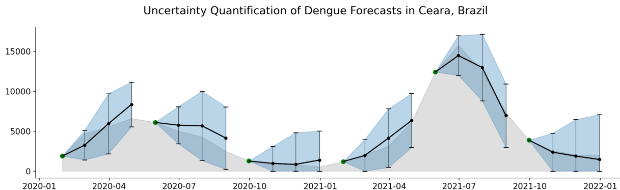
Figure 10: Demonstration of uncertainty quantification interval algorithm in Ceara, Brazil. The green points indicate the reference months m , and each set of subsequent three black points marks the 1-, 2-, and 3-month ahead point forecasts. The error bars corresponding to each point forecast quantify our 95% approximate predictive intervals. The blue cones emphasize how the uncertainty in our forecasts evolves over forecast horizon. The grey silhouette shows the ground truth reported dengue case counts.
