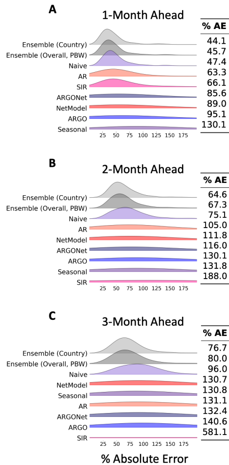
Figure 13: Overall error distributions for standard individual and ensemble models across all 187 tested locations. (A) - (C) Ridgeline plots show percent absolute error distributions at the 1-month, 2-month, and 3-month horizons, respectively. Side tables record the mean percent absolute error incurred.
