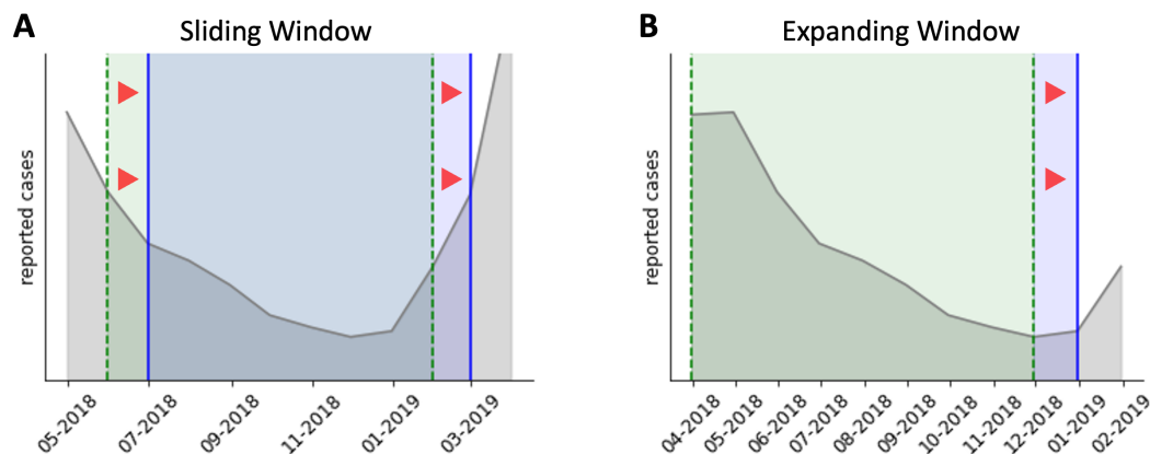
Figure 8: Schematics of model-fitting techniques. (A) Sliding window model-fitting. (B) Expanding window model-fitting.
