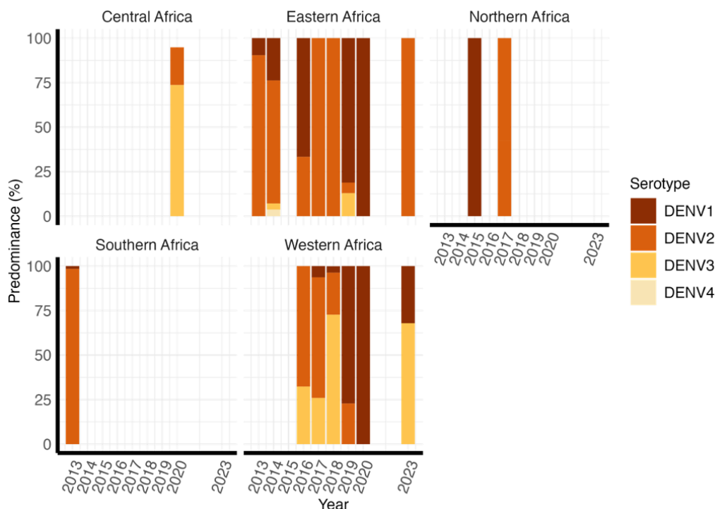
34 35 Figure 4. Spatiotemporal distribution of DENV serotypes in Africa based on the data 36 available from 2013 to 2023.
