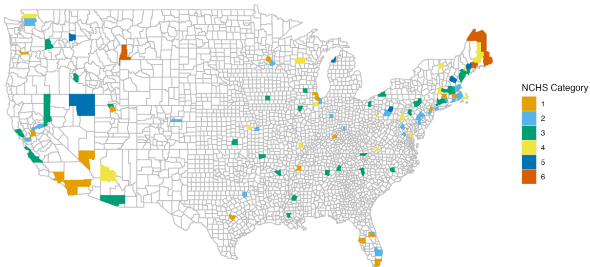
4 5 Figure 1: This shows geographic location and NCHS urbanicity category for the 107 counties included in the 6 analysis.
