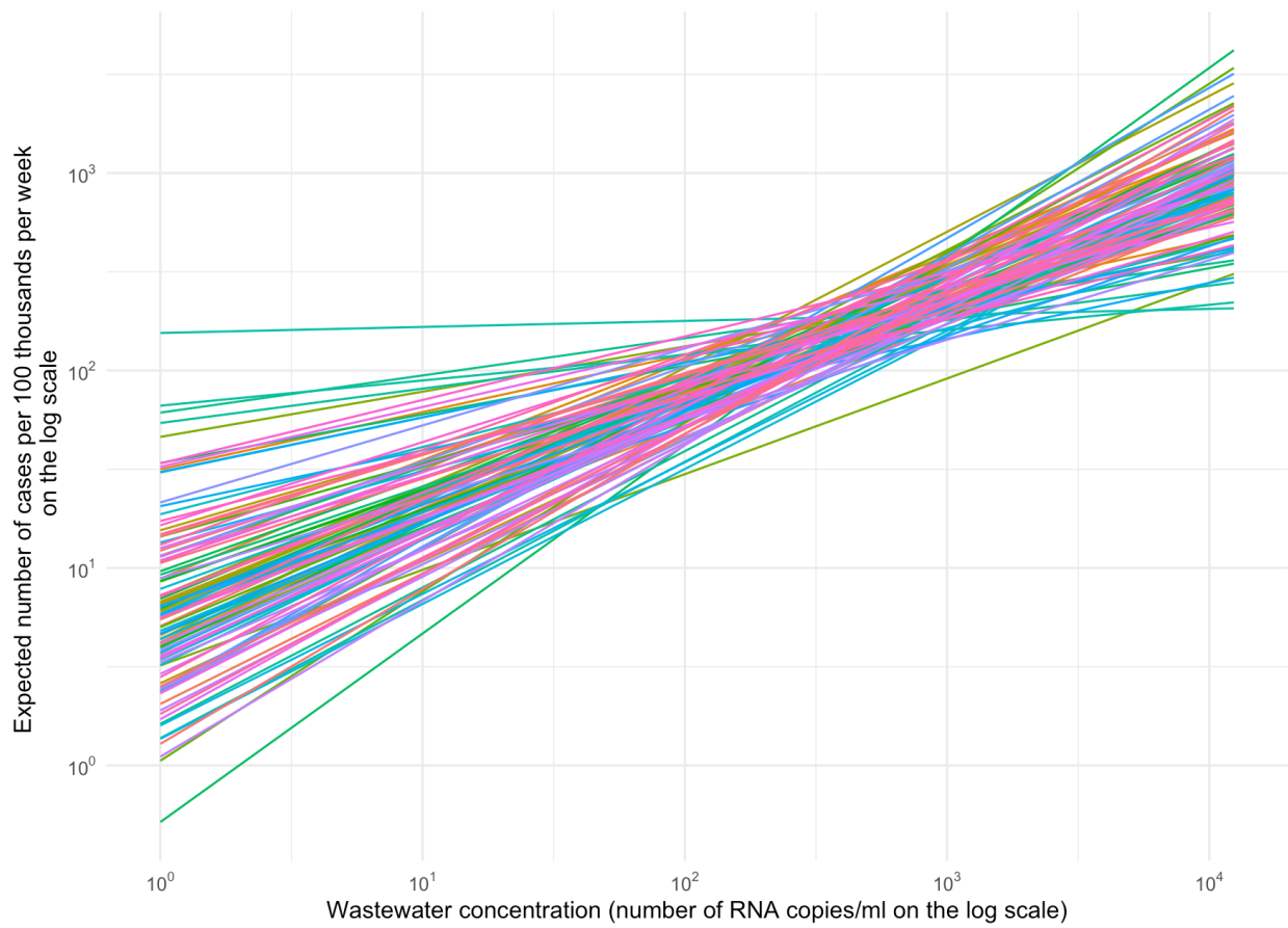
1 2 Figure 5: Estimated relationship between wastewater concentration and mean weekly cases per 100 3 thousand people for each county.
