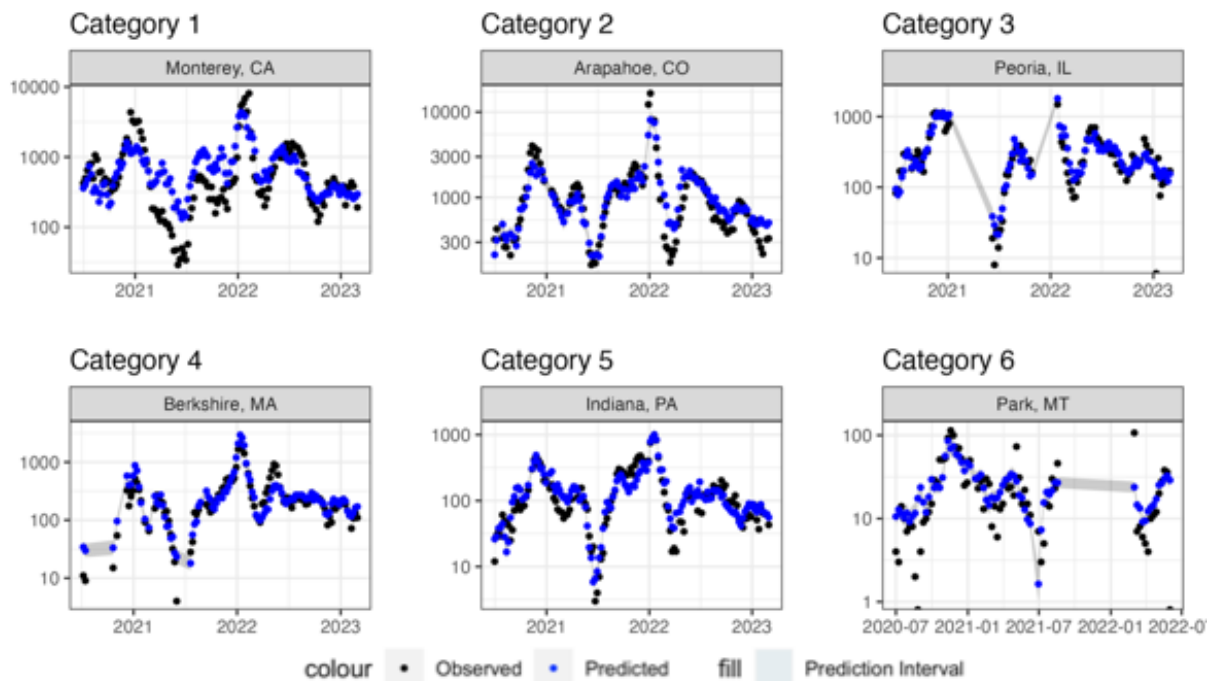
3 4 Figure 2: Comparison of observed and predicted COVID-19 case counts for a select group of counties within 5 each urban-rural category as defined by the National Center for Health Statistics (NCHS).
