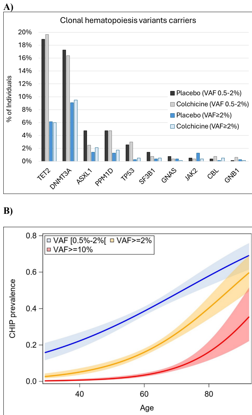
Figure 1. Prevalence of clonal hematopoiesis variant carriers, based on the mutation with the highest variant allele fraction (VAF) value in the first sample collected. A. Percentage of carrier individuals by gene, group, and VAF category. B. Prevalence of variant carriers of any gene mutation by age.
