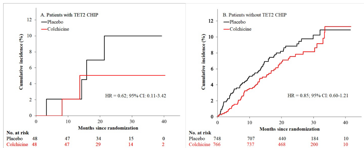
Figure 2. Cumulative incidence curves of the cardiovascular composite endpoint (cardiovascular death, resuscitated cardiac arrest, myocardial infarction, stroke, urgent hospitalization for angina requiring coronary revascularization, or any coronary revascularization) in the colchicine group (red) and the placebo group (black), in a time-to-event analysis, for patients A. with TET2 CHIP mutations and B. without TET2 CHIP mutations.
