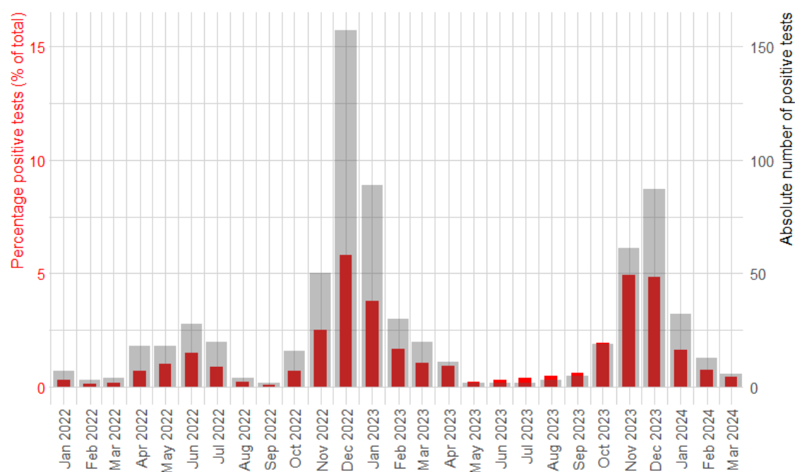
Figure 1 Epidemiology of respiratory syncytial virus (RSV) during the study period for all hospitals combined. The red bars define the percentage of positive RSV tests as a fraction of all performed RSV tests (scale on the left). The grey bars define the absolute number of positive RSV tests (scale on the right).
