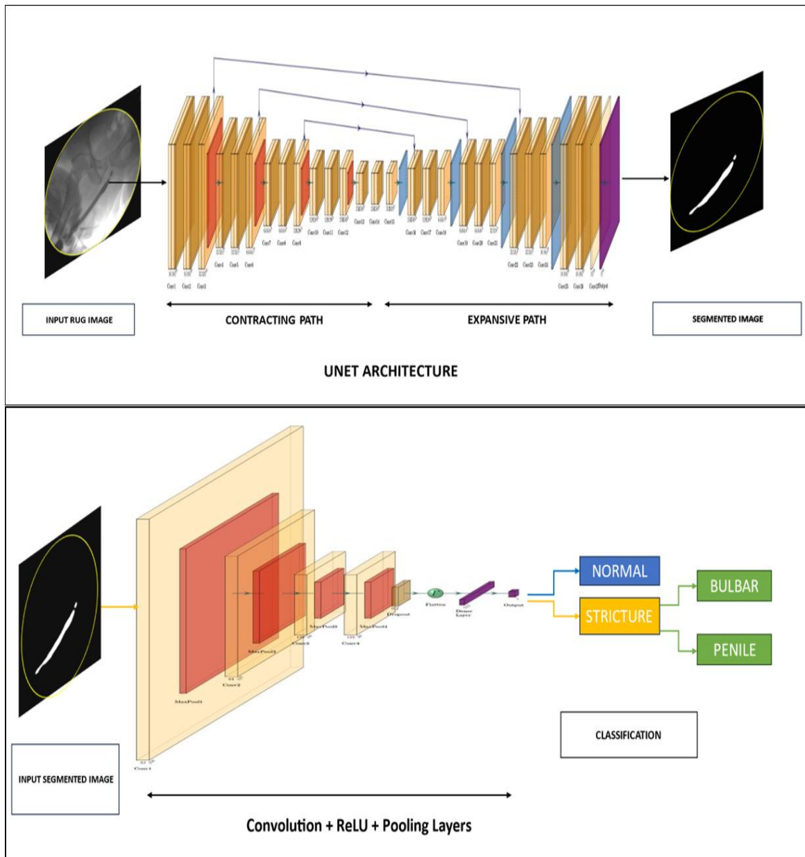
Figure 1: Overall model summary – an input RUG image is fed to the UNET architecture which outputs the segmented image. The resultant image is then given as an input to the classification model which will eventually classify the given image as strictured or normal. Further the strictured image was sub classified into bulbar and penile stricture.
