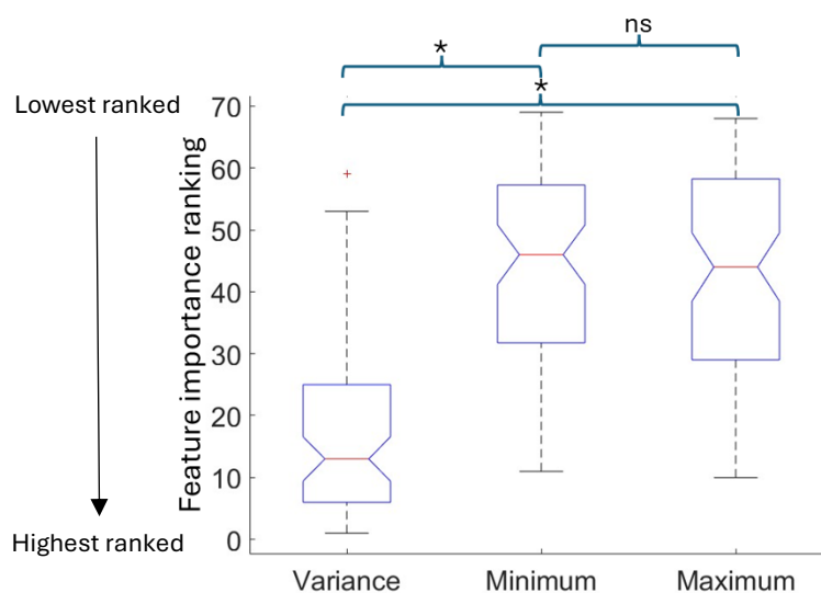
Figure 3. Comparison of the mean importance ranking of variance, minimum and maximum features. Features are ranked from 1 (highest importance) to 69 (lowest importance). The mean feature importance ranking for the variance features was significantly better than the mean rankings for minimum and maximum features (one-way ANOVA, *p < 0.005 ). Whiskers indicate the interquartile range, the upper and lower edges of the boxes represent the 75th and the 25th percentile of the distribution, respectively, and the red middle line represents the median of the distribution.
