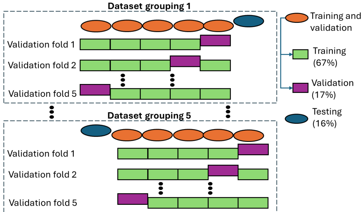
Figure 1. Dystonia diagnostic model training, validation, and testing. The full video dataset is divided into different subsets for training (2/3 of the dataset), validation (1/6 of the dataset), and testing (1/6 of the dataset) in each of 5 different dataset groupings of the full dataset. Within each dataset grouping, training and validation occurs 5 times, using different subsets for training and validation each time.
