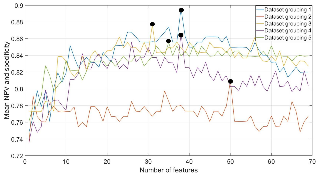
Figure 4. The mean of NPV and specificity of ML models when trained on different numbers of top-ranked features. The black points denote the best performing model for each of the five dataset groupings of the full dataset. The x-axis represents the number of features used for training and validation. For instance, a value of 50 on the x-axis indicates that the top 50 features, according to their importance, were used for training and validating the models. The y-axis represents the mean validation NPV and specificity of the best-performing ML model (out of 4664 models) when trained on the selected number of features.
