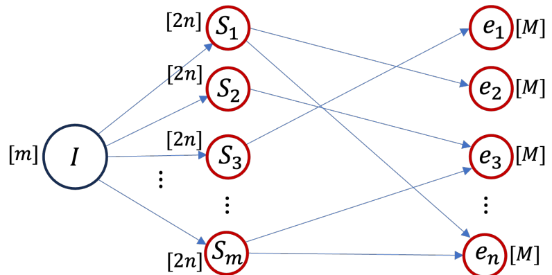
Fig 1. The instance of MAXCASESAVERTED and MAXPEAKSREDUCED is a graph G constructed from the given instance (\mathcal{C} = (S_1, S_2, \dots, S_m), \mathcal{U} = (e_1, e_2, \dots, e_n), k) of MAX k -SI. Each node represents a subpopulation, with the size of the subpopulation shown in square brackets next to it. The directed edges permit 1 unit flow. The unit flows from nodes S_j to e_i encode non-membership. For example, the flow from S_1 to e_2 implies that e_2 \notin S_1 .
