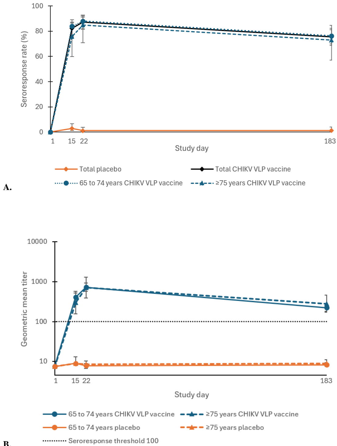
Figure 2. A. Seroresponse Rate and B. Geometric Mean Titers for CHIKV Serum Neutralizing Antibodies by Visit and by Age Group (Immunogenicity Evaluable Population).
