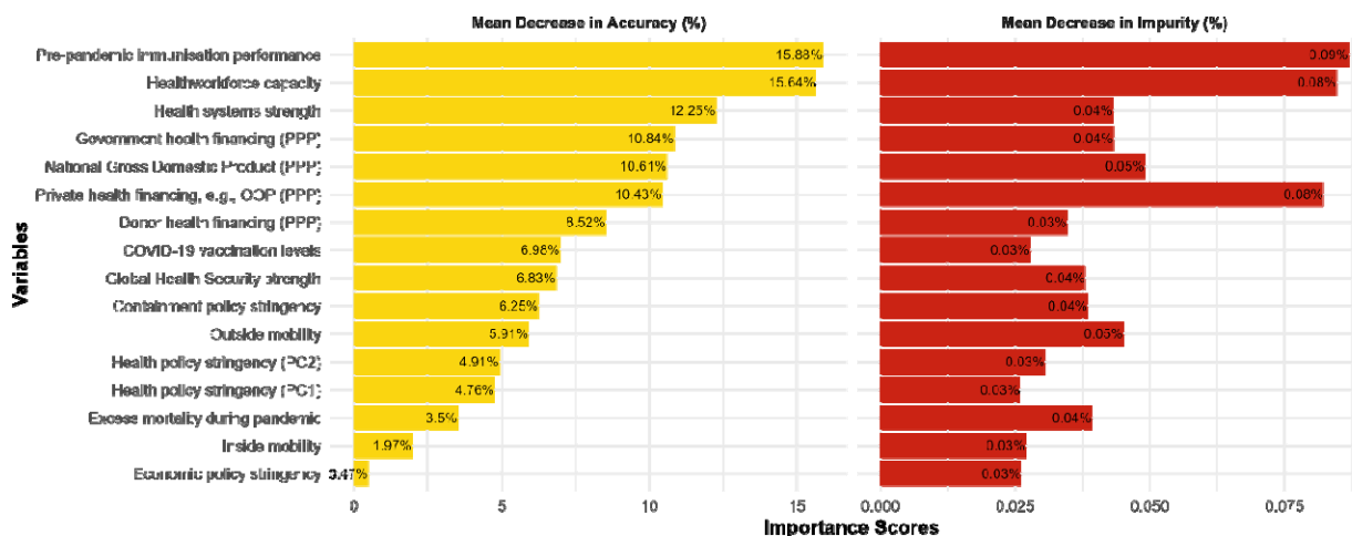
Figure 2. Variable importance scores from the Random Forest regression. The Mean Decrease in Accuracy (MDA) is calculated by permuting the values of each variable and measuring the resulting decrease in the model's accuracy. Mean Decrease in Impurity (MDI) measures the total reduction in impurity (e.g., Gini impurity) brought by a variable across all trees in the forest. It reflects the variable's ability to split the data into more homogeneous nodes. Both MDA and MDI scores are relative to a given model, and higher values indicate that a variable is more important (MDA) and is better splitting the data effectively (MDI).
